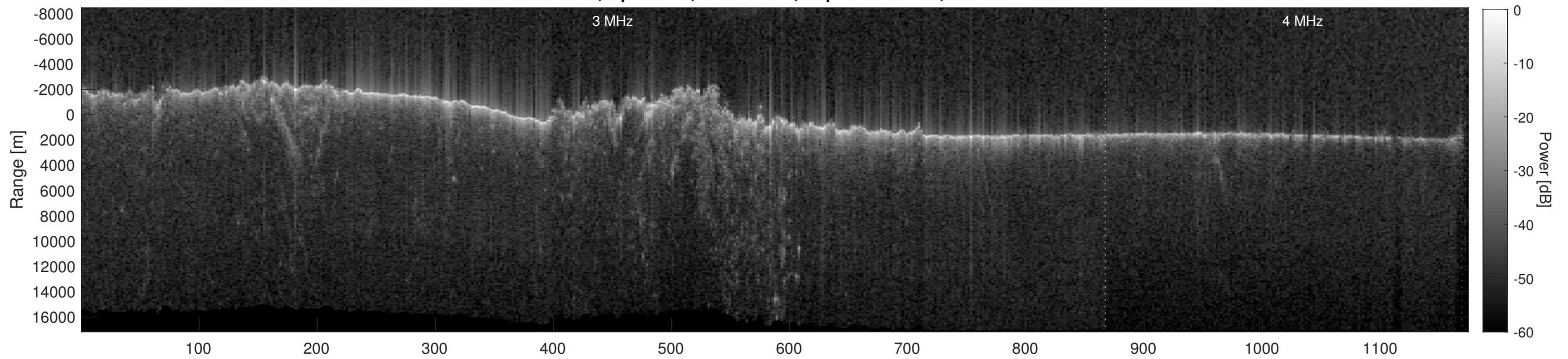
Orbit 5959, Depth-Corrected Cluttergram
