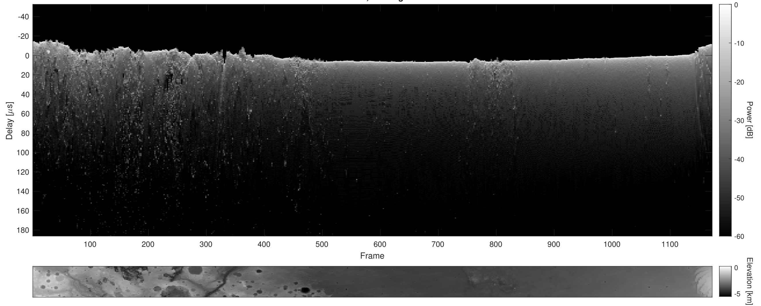
Orbit 5960, Cluttergram
