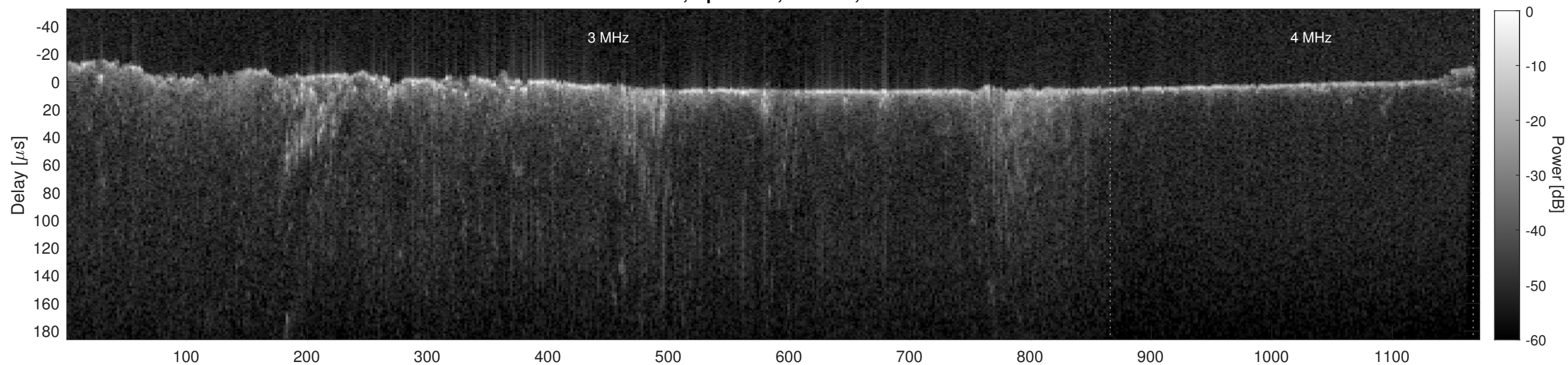
Orbit 5960, Cluttergram
