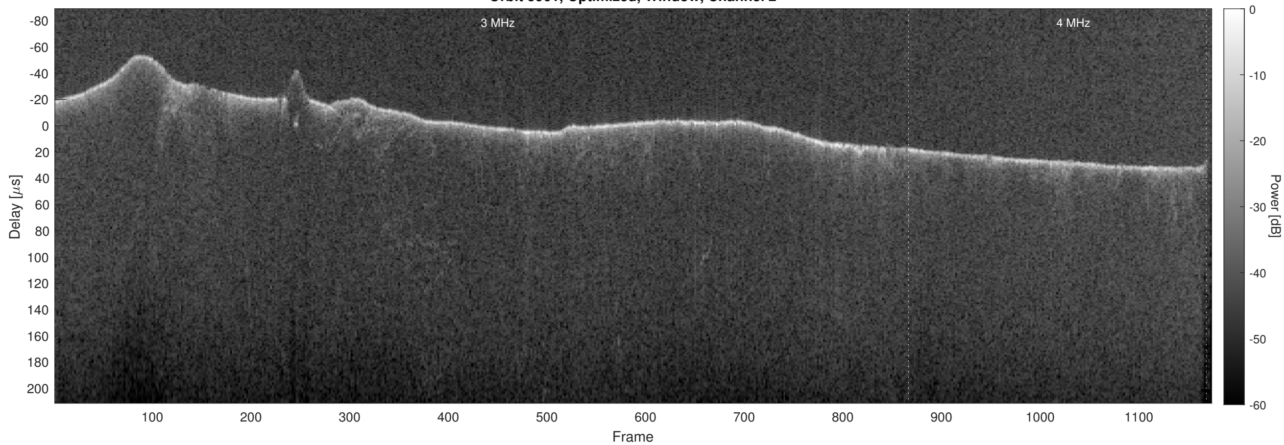
Orbit 5961, Optimized, Window, Channel 2
