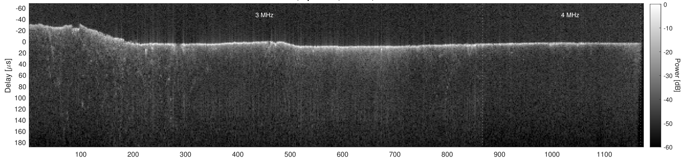
Orbit 5962, Cluttergram
