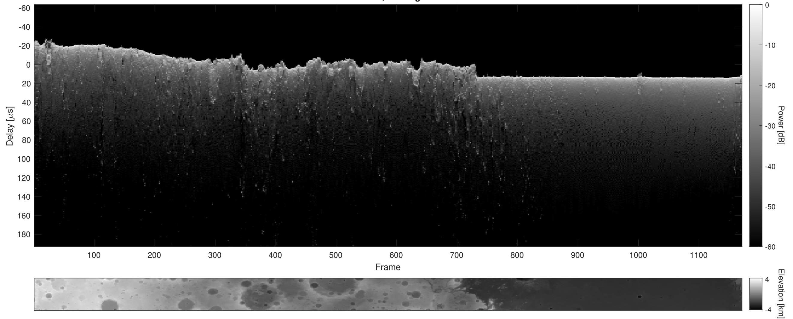
Orbit 5963, Cluttergram
