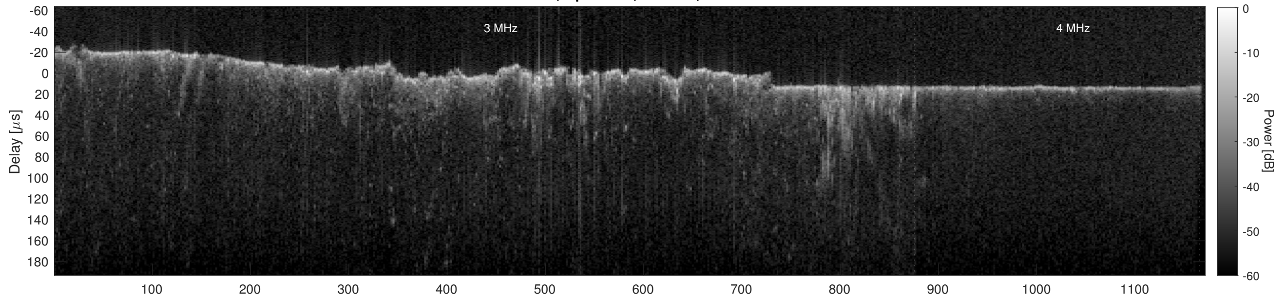
Orbit 5963, Cluttergram
