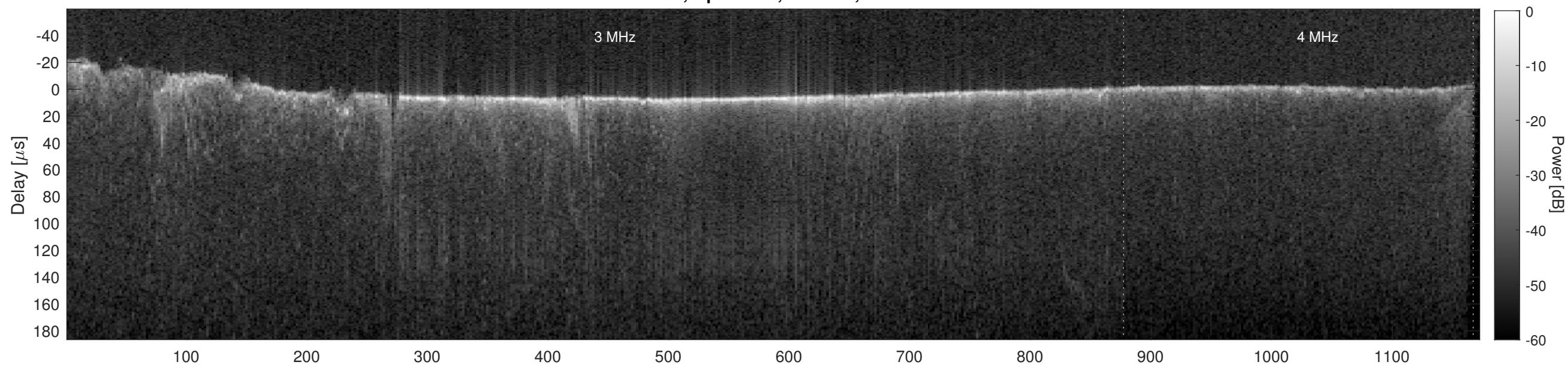
Orbit 5965, Cluttergram
