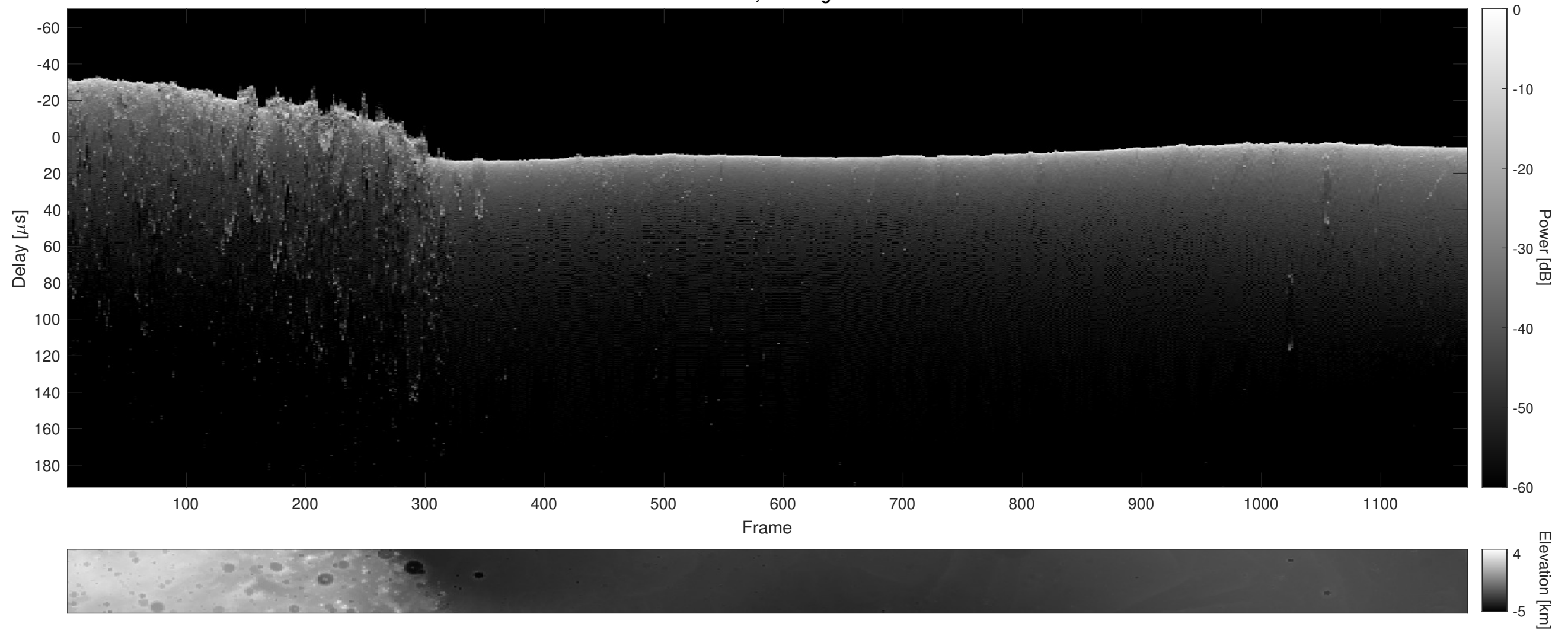
Orbit 5966, Cluttergram
