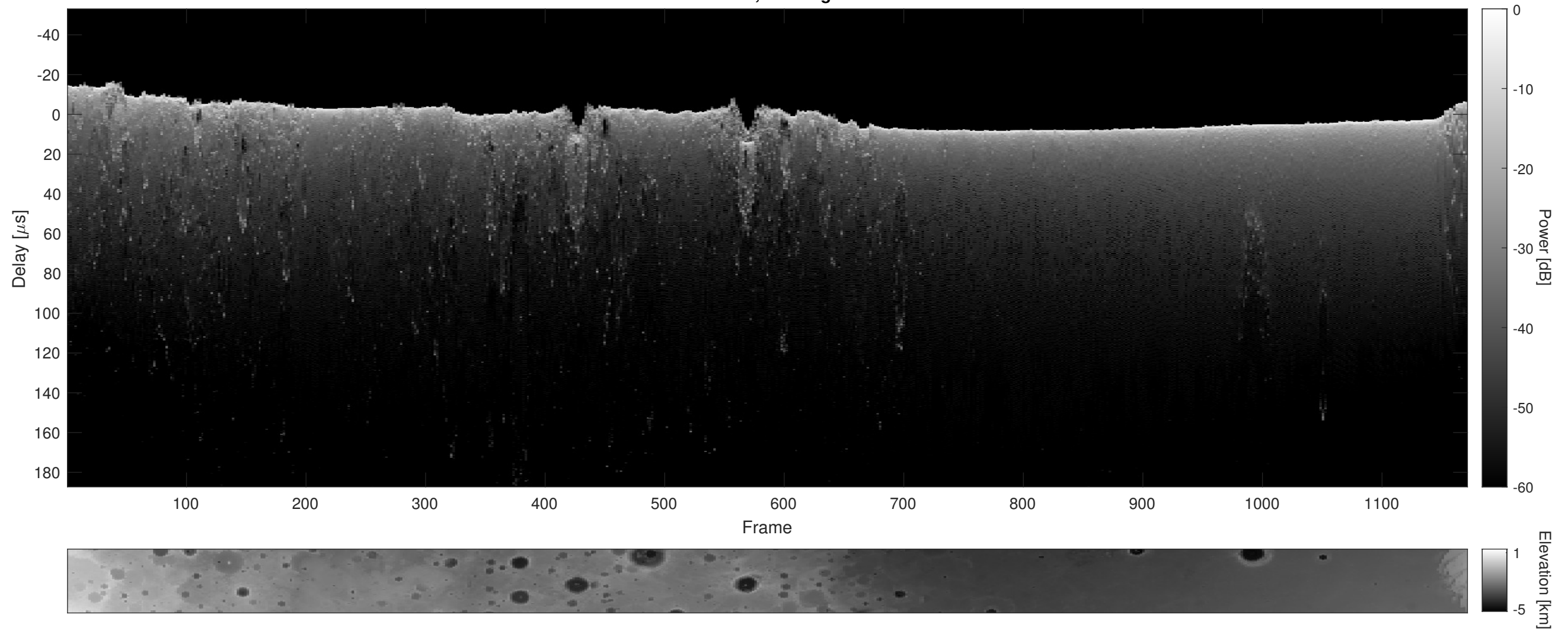
Orbit 5967, Cluttergram
