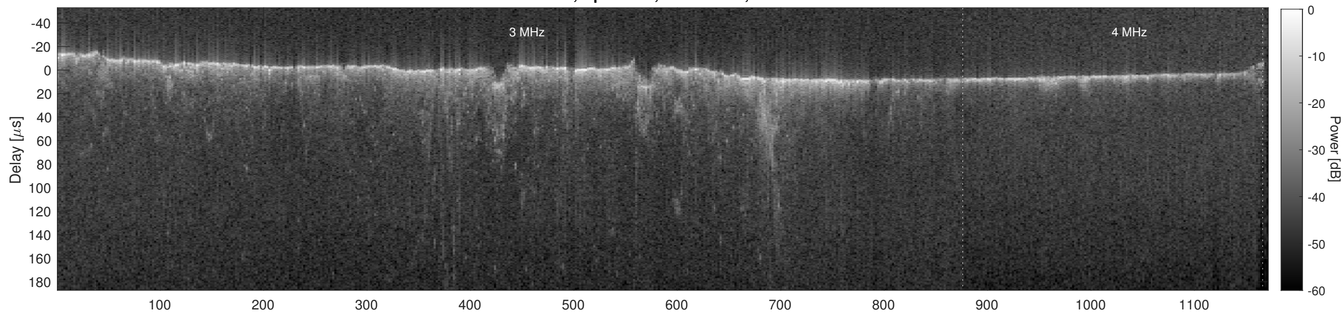
Orbit 5967, Cluttergram
