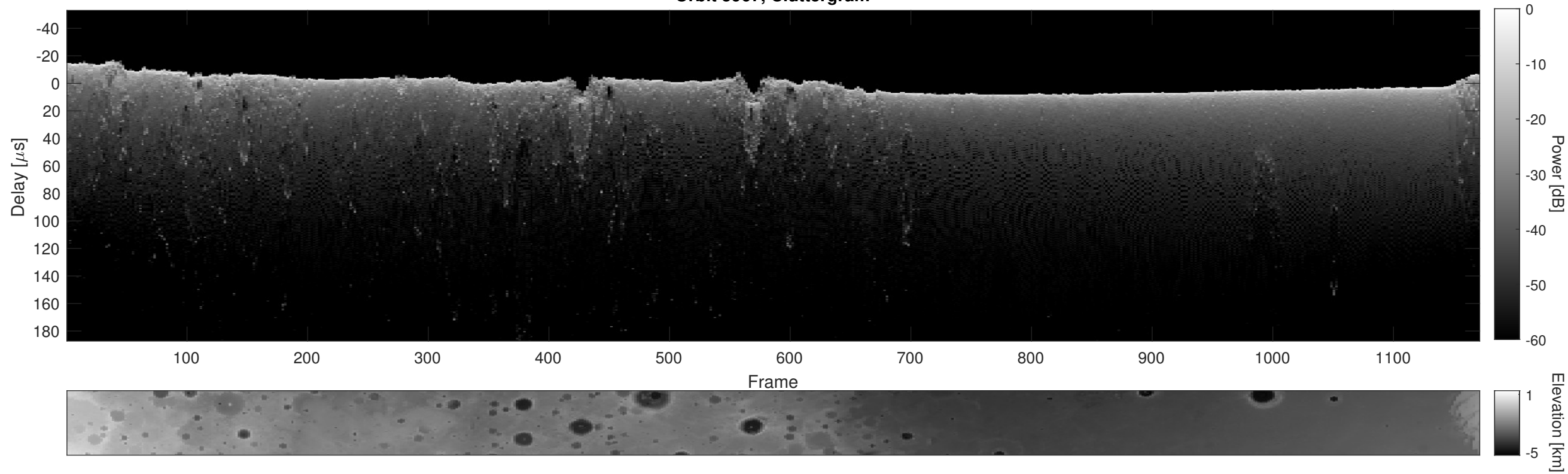
Orbit 5967, Cluttergram
