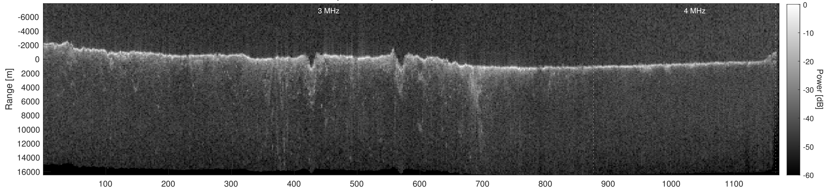
Orbit 5967, Depth-Corrected Cluttergram
