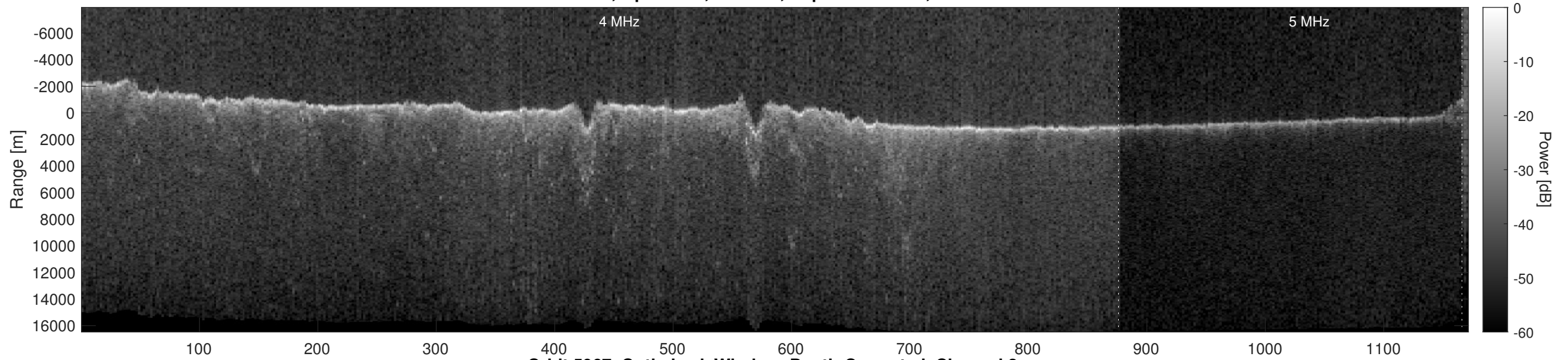
Orbit 5967, Optimized, Window, Depth-Corrected, Channel 2
