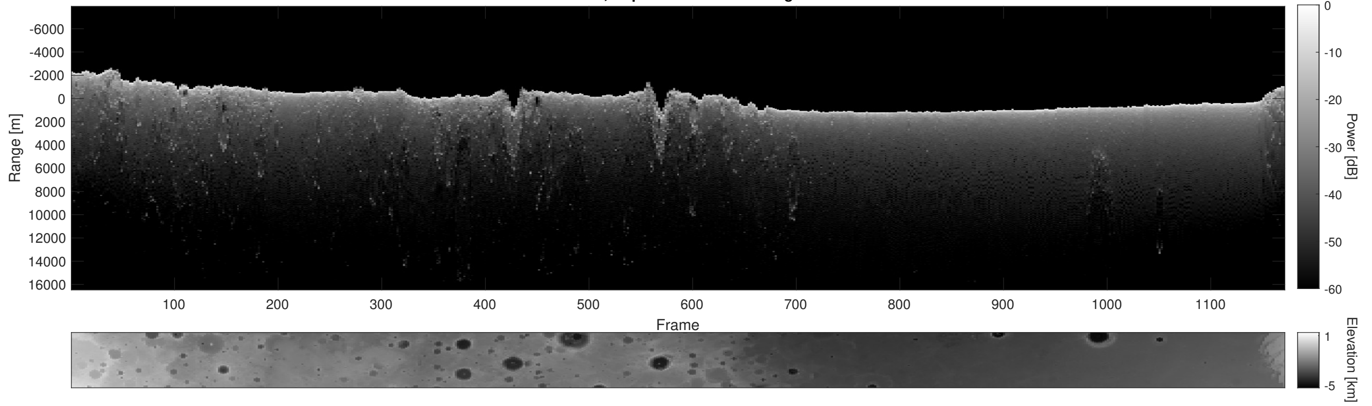
Orbit 5967, Depth-Corrected Cluttergram
