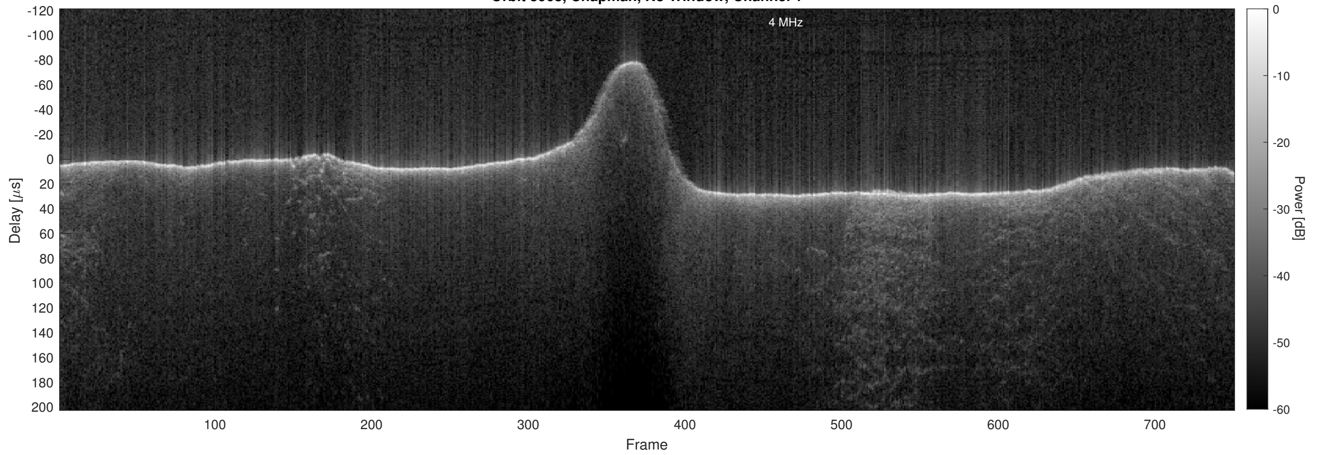
Orbit 5968, Chapman, No Window, Channel 2
