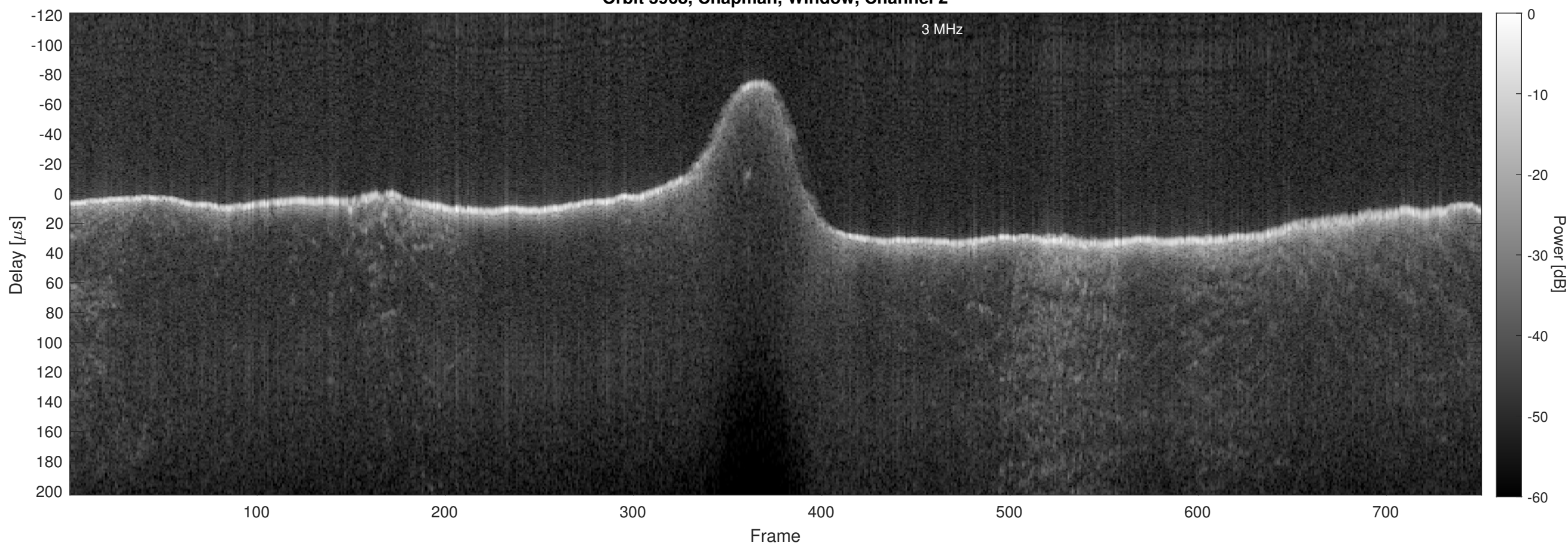
Orbit 5968, Chapman, Window, Channel 2
