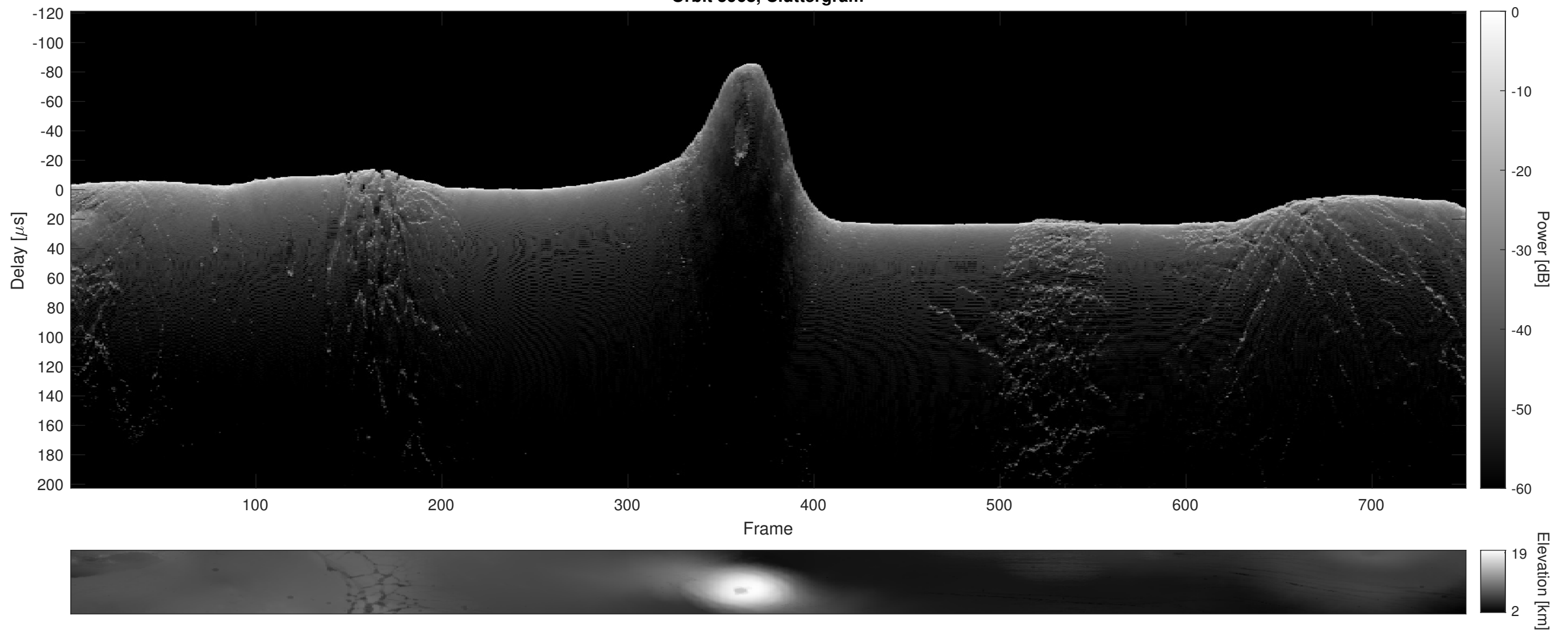
Orbit 5968, Cluttergram
