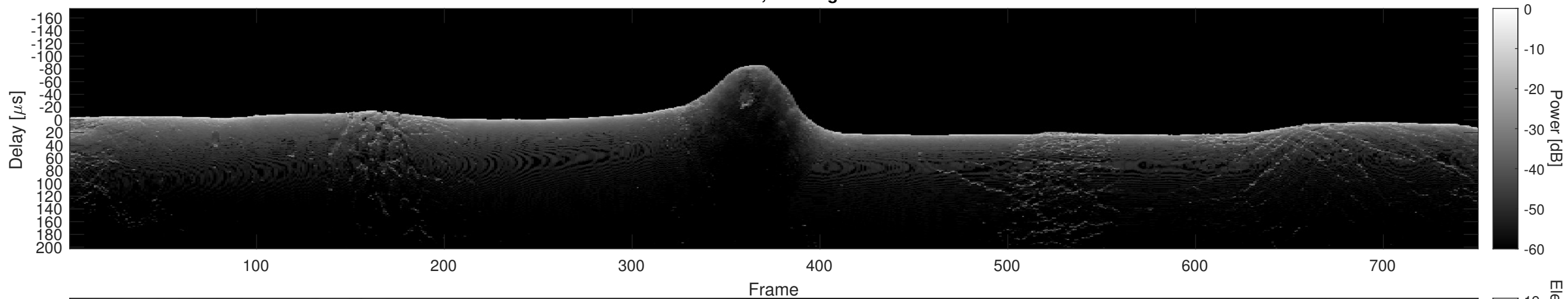
Orbit 5968, Cluttergram
