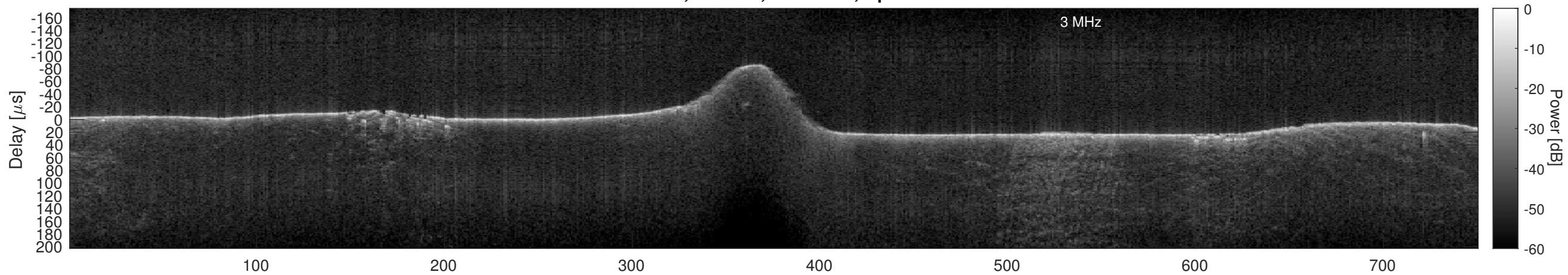
Orbit 5968, Cluttergram
