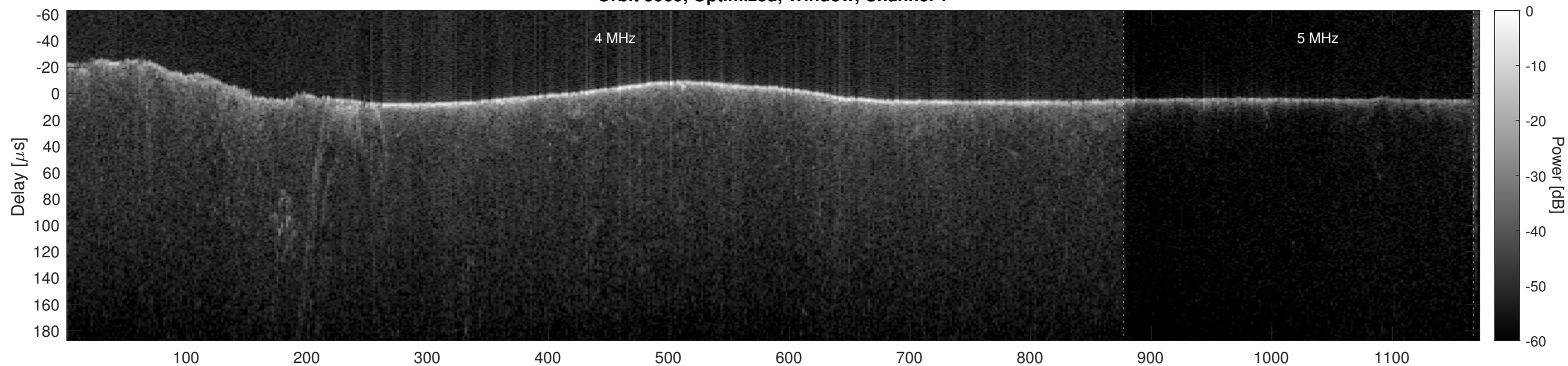
Orbit 5969, Optimized, Window, Channel 2
