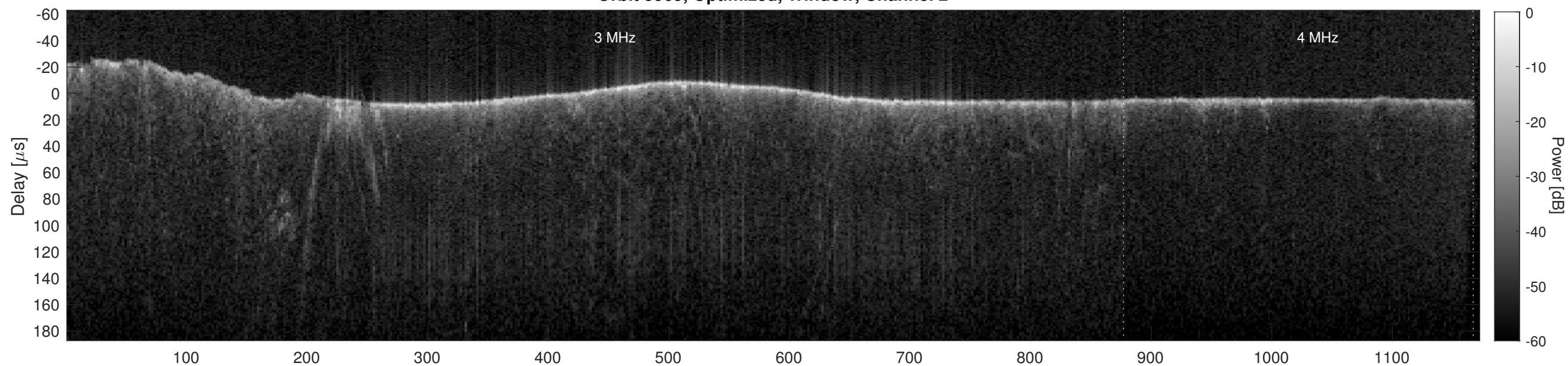
Orbit 5969, Cluttergram
