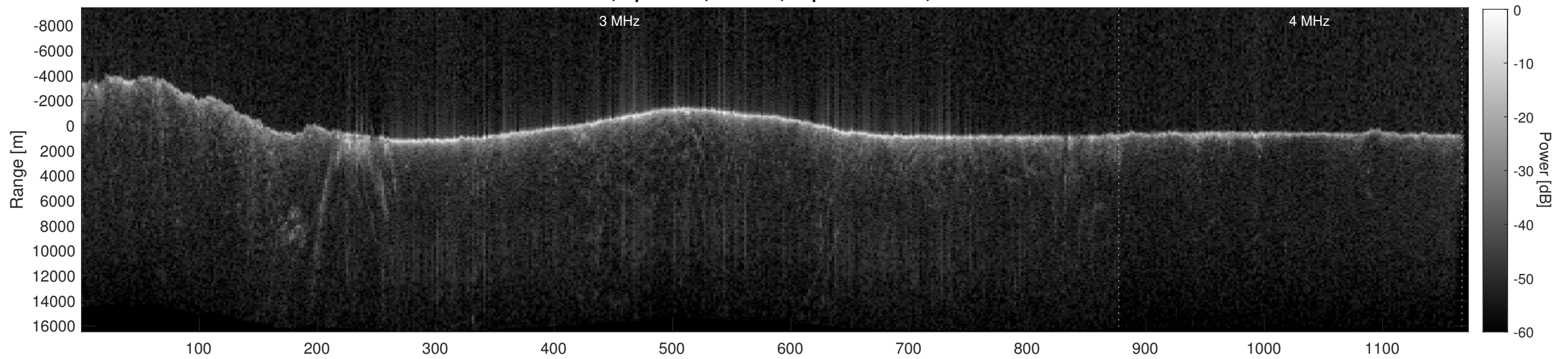
Orbit 5969, Depth-Corrected Cluttergram
