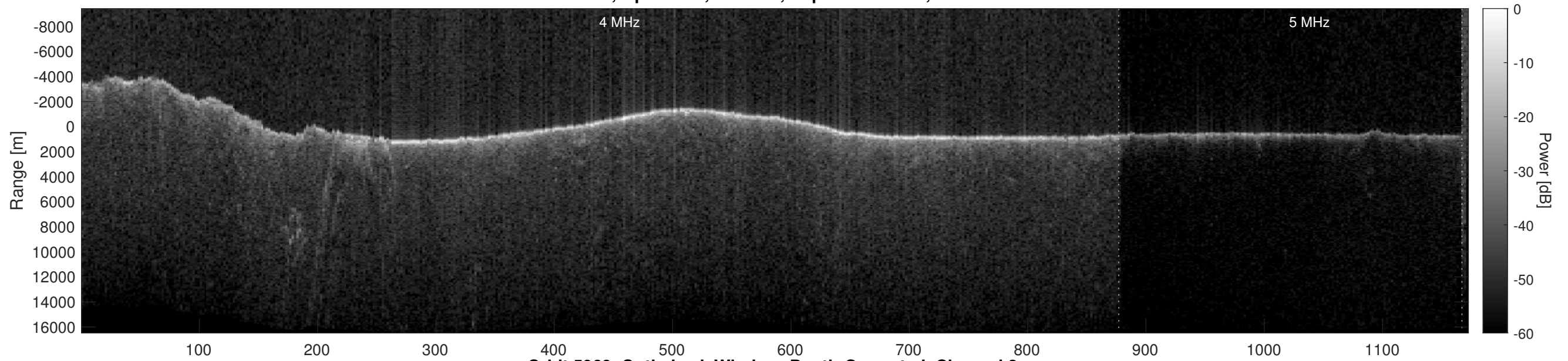
Orbit 5969, Optimized, Window, Depth-Corrected, Channel 2
