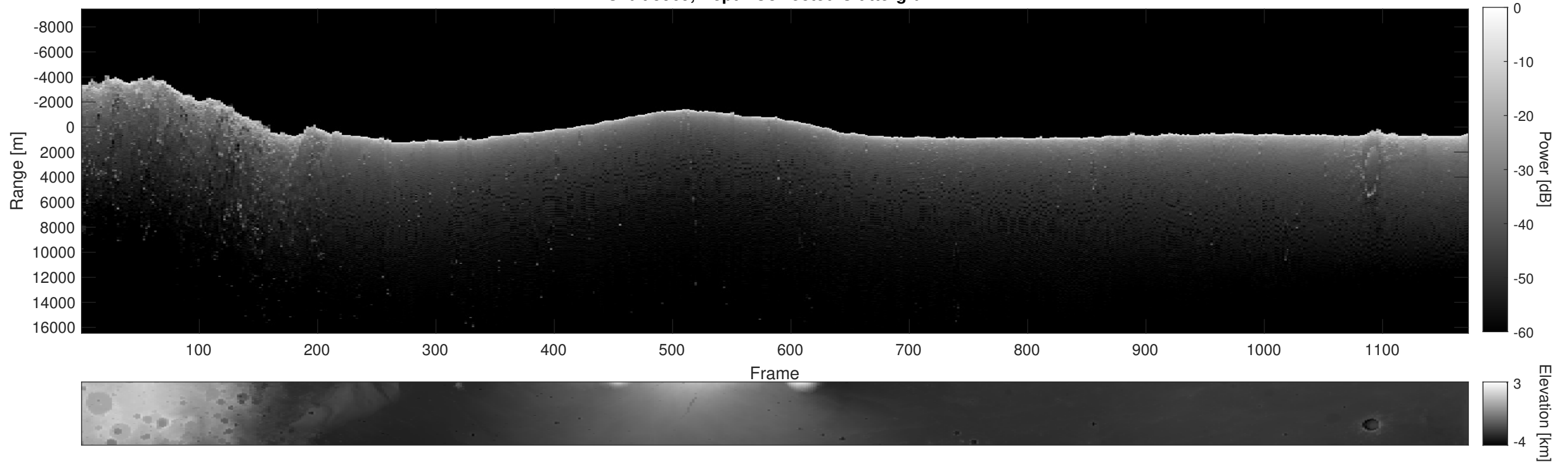
Orbit 5969, Depth-Corrected Cluttergram
