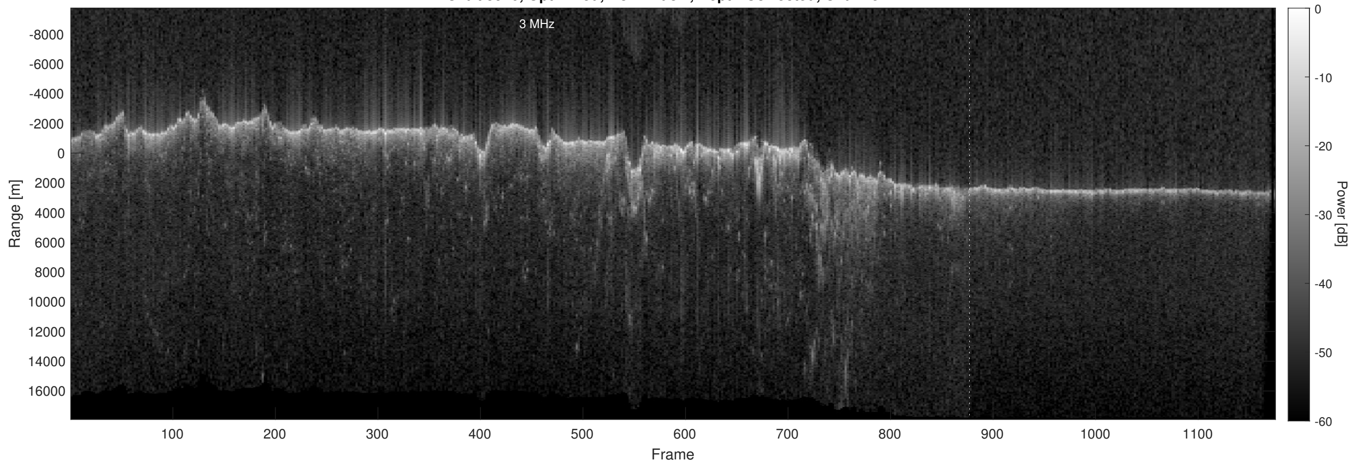
Orbit 5970, Optimized, No Window, Depth-Corrected, Channel 2
