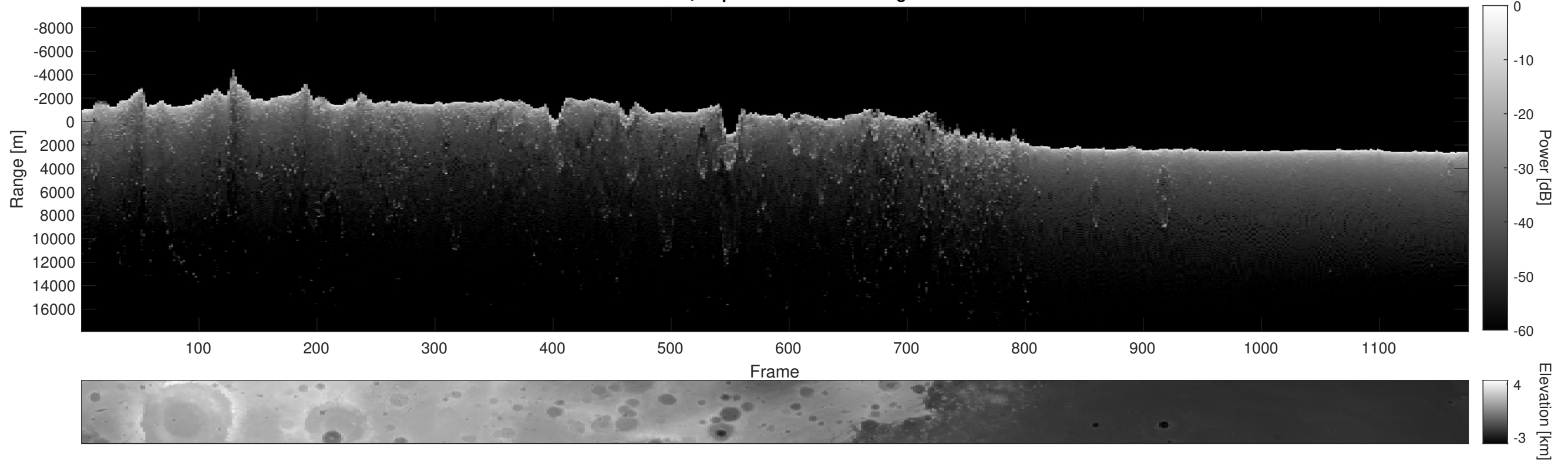
Orbit 5970, Depth-Corrected Cluttergram
