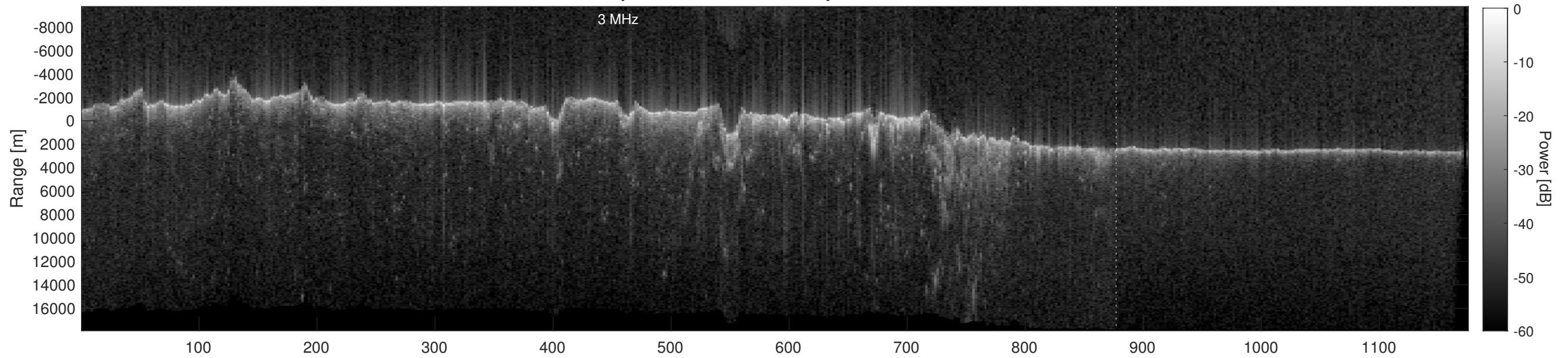
Orbit 5970, Depth-Corrected Cluttergram
