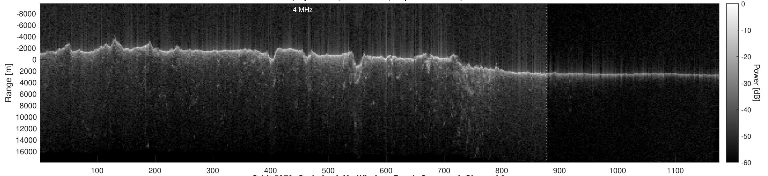
Orbit 5970, Optimized, No Window, Depth-Corrected, Channel 2
