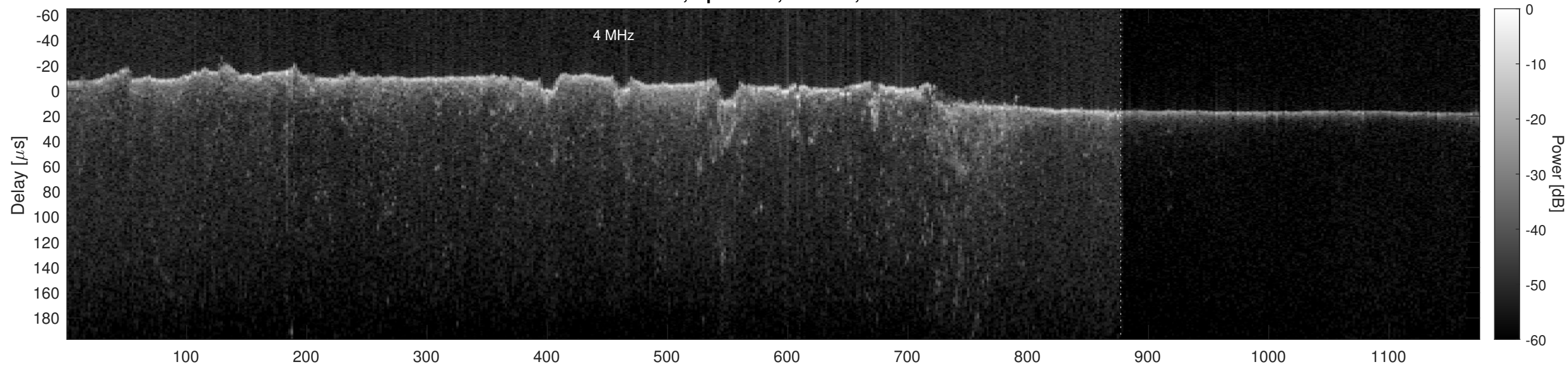
Orbit 5970, Optimized, Window, Channel 2
