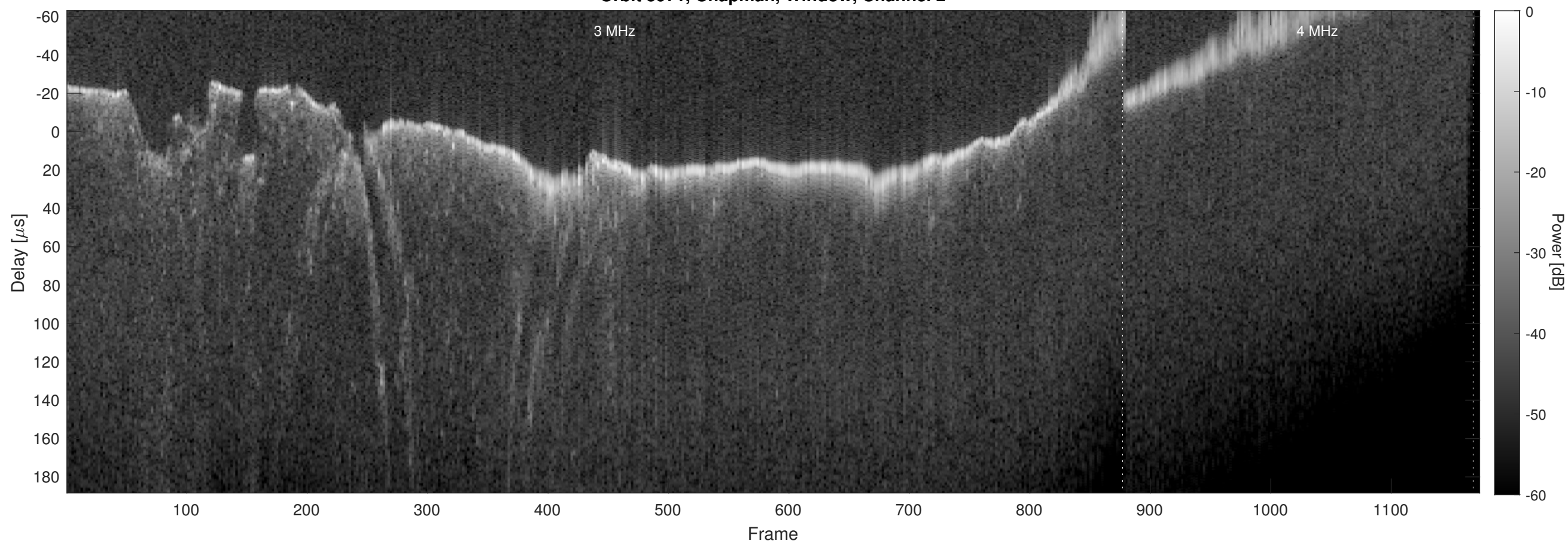
Orbit 5971, Chapman, Window, Channel 2
