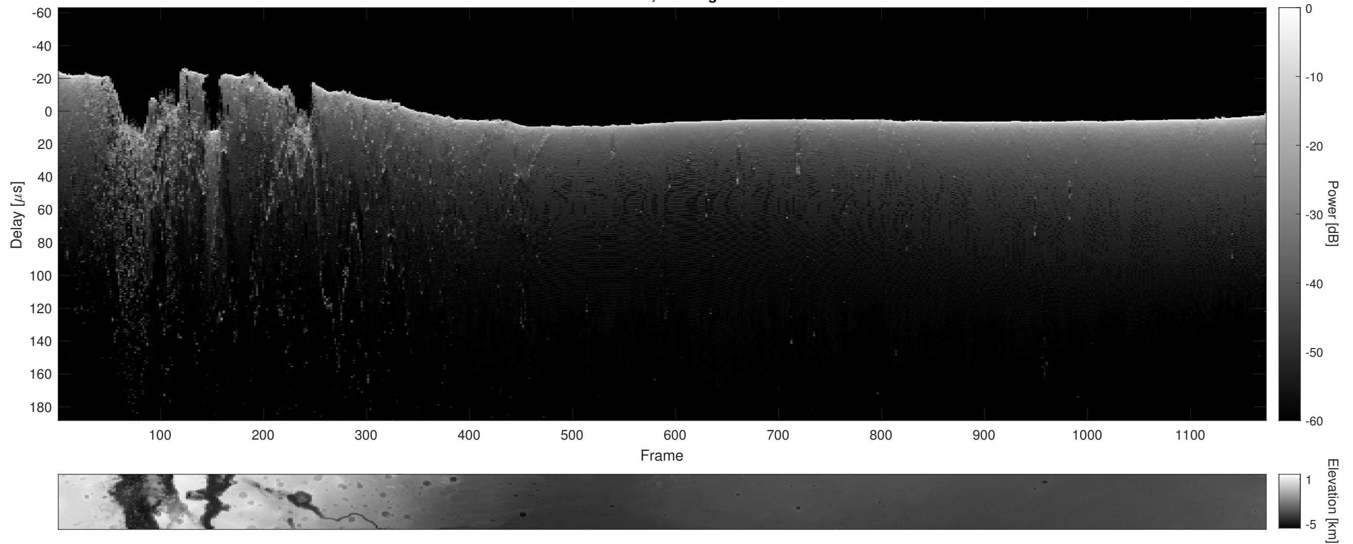
Orbit 5971, Cluttergram
