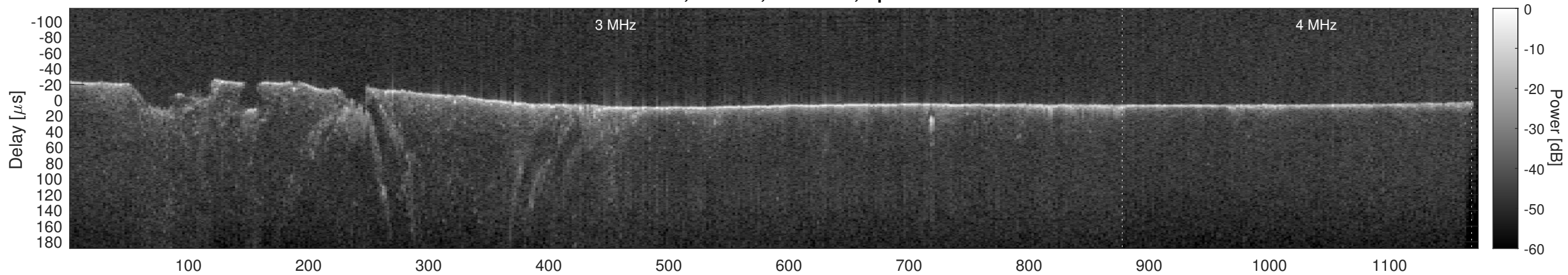
Orbit 5971, Cluttergram
