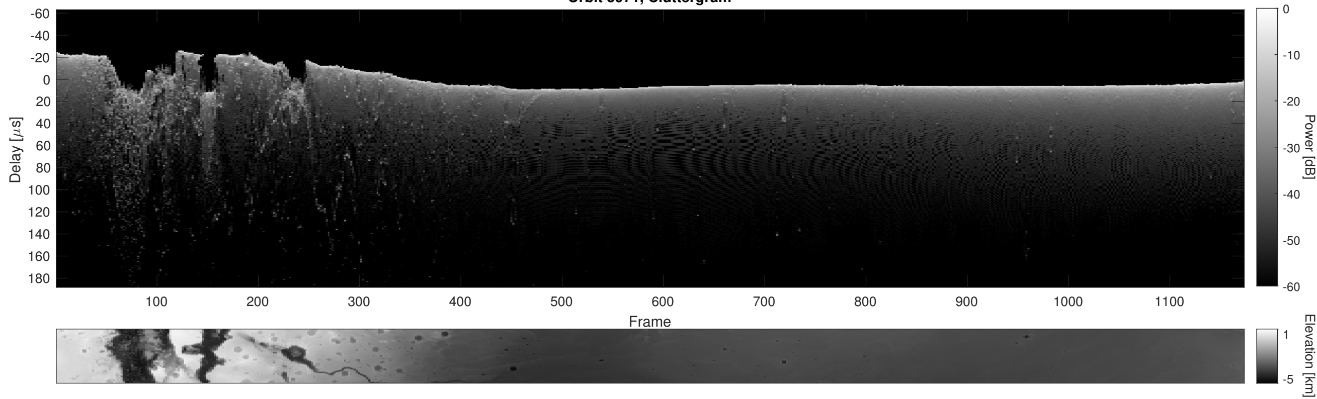
Orbit 5971, Cluttergram
