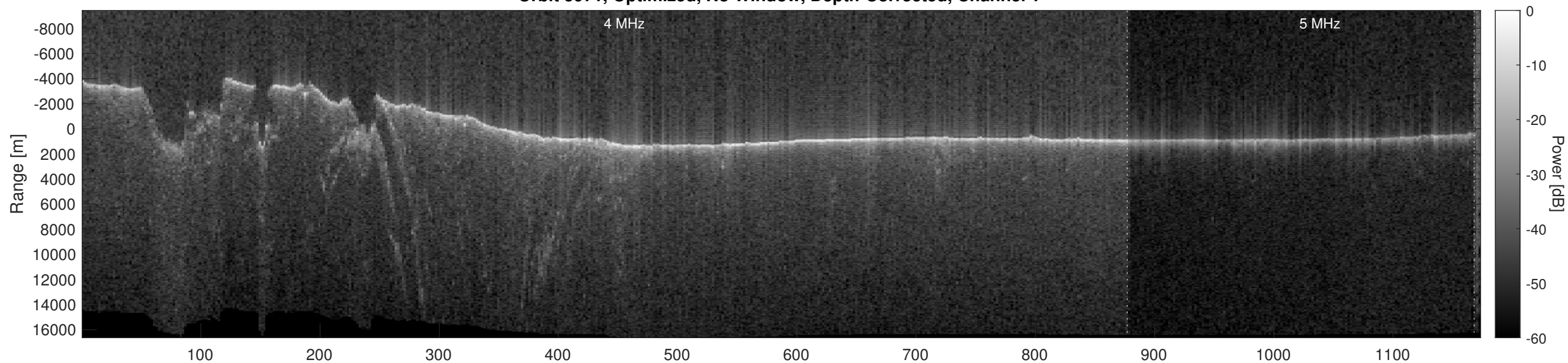
Orbit 5971, Optimized, No Window, Depth-Corrected, Channel 2
