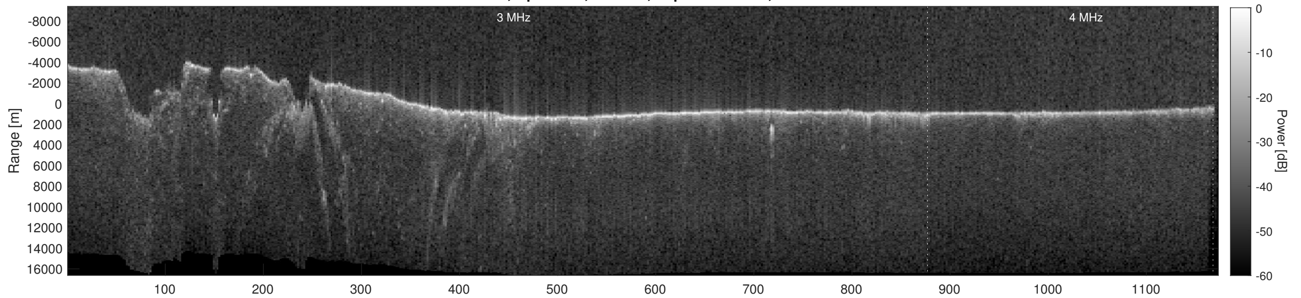
Orbit 5971, Depth-Corrected Cluttergram
