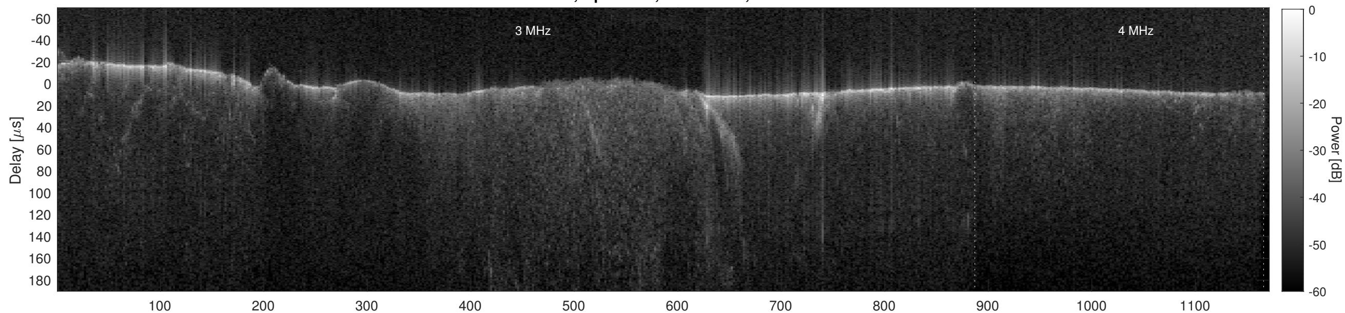
Orbit 5972, Cluttergram
