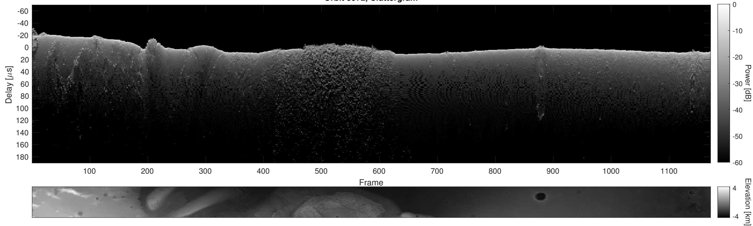
Orbit 5972, Cluttergram
