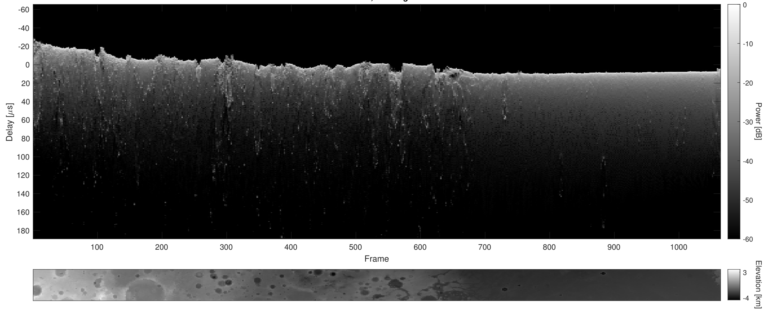
Orbit 5974, Cluttergram
