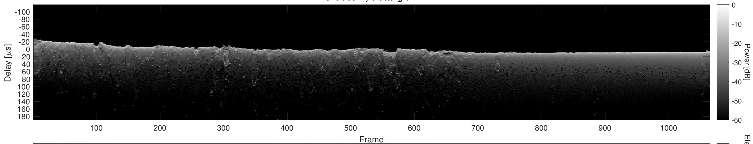
Orbit 5974, Cluttergram
