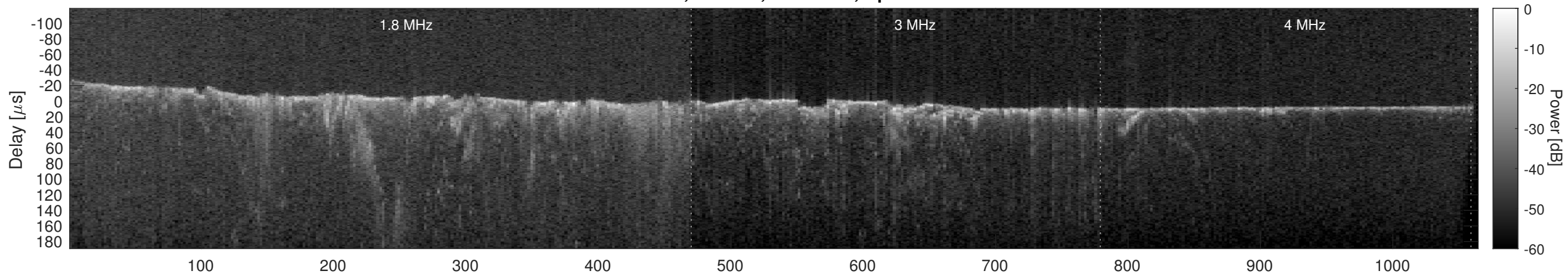
Orbit 5974, Cluttergram
