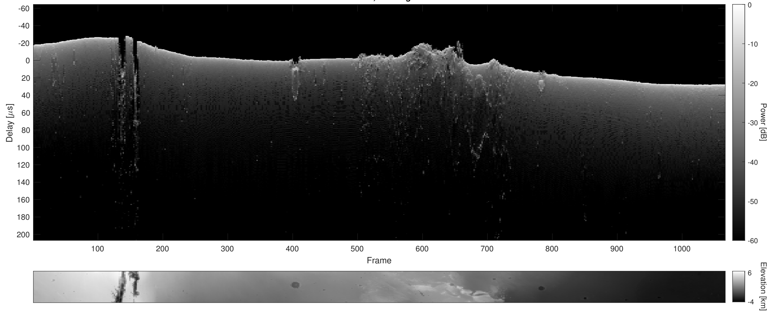
Orbit 5975, Cluttergram
