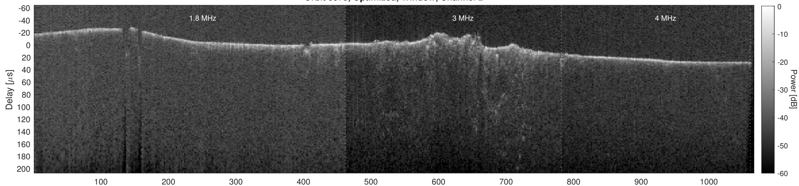
Orbit 5975, Cluttergram
