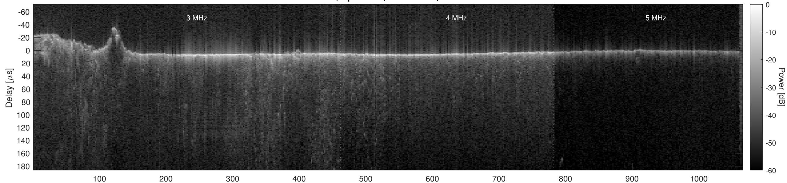
Orbit 5976, Optimized, No Window, Channel 2
