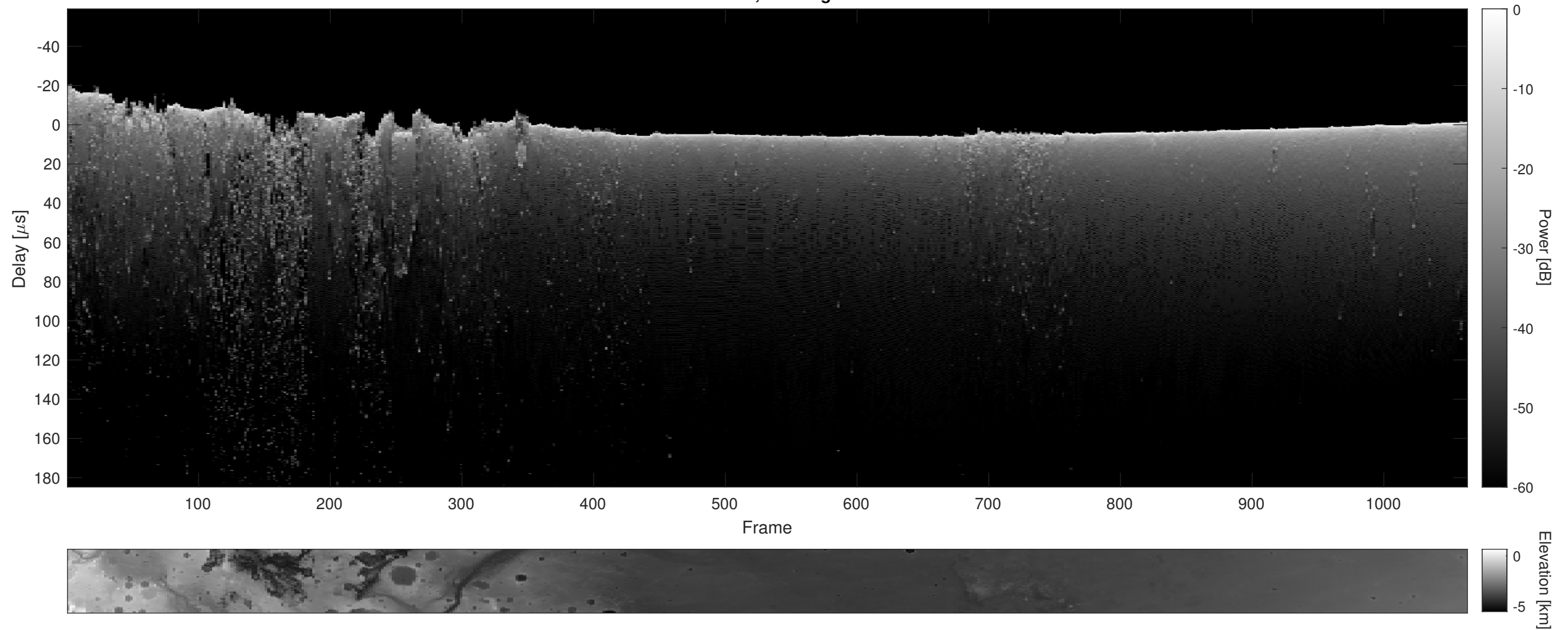
Orbit 5978, Cluttergram
