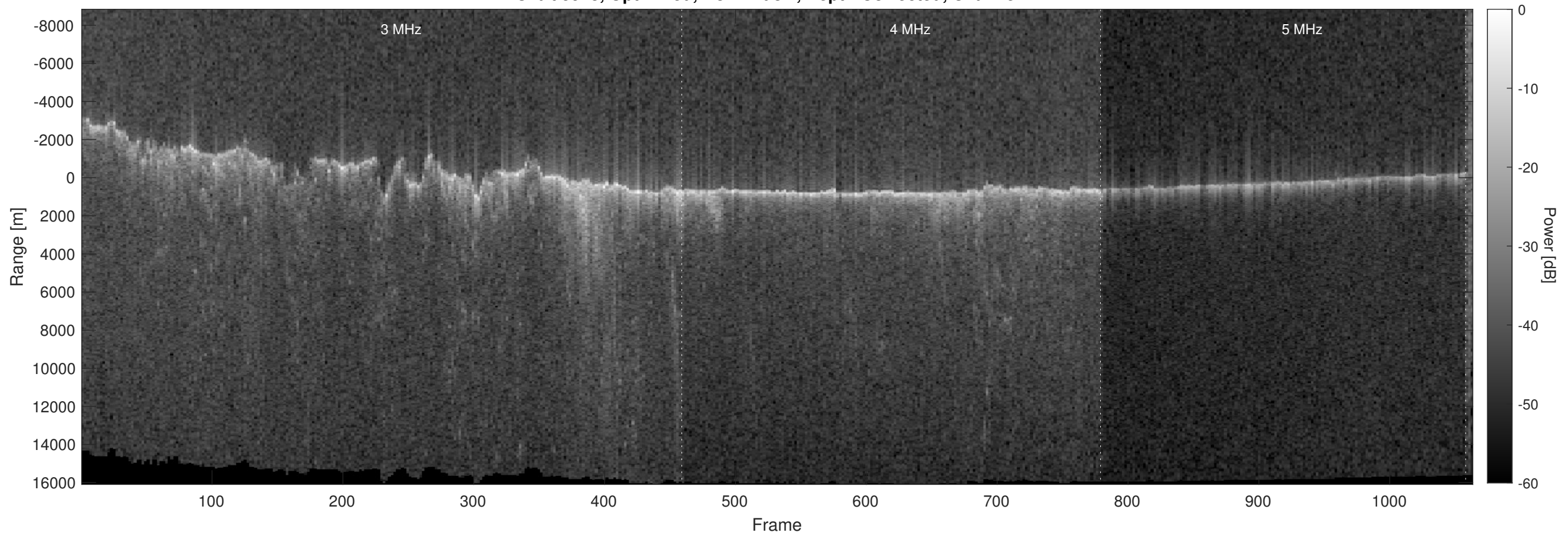
Orbit 5978, Optimized, No Window, Depth-Corrected, Channel 2
