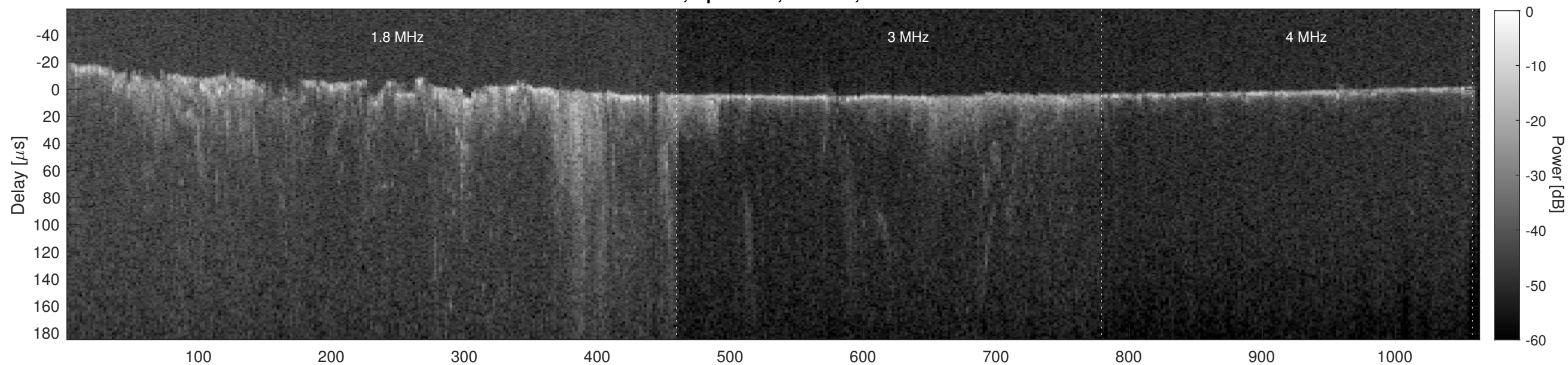
Orbit 5978, Cluttergram
