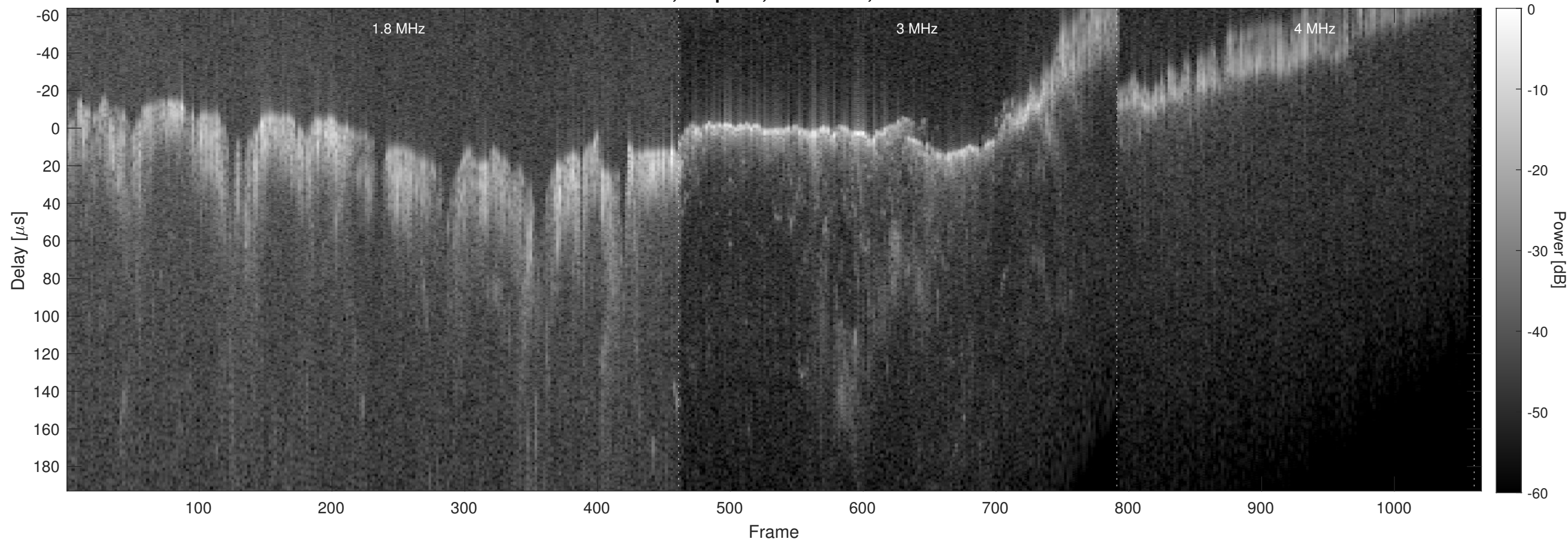
Orbit 5981, Chapman, No Window, Channel 2
