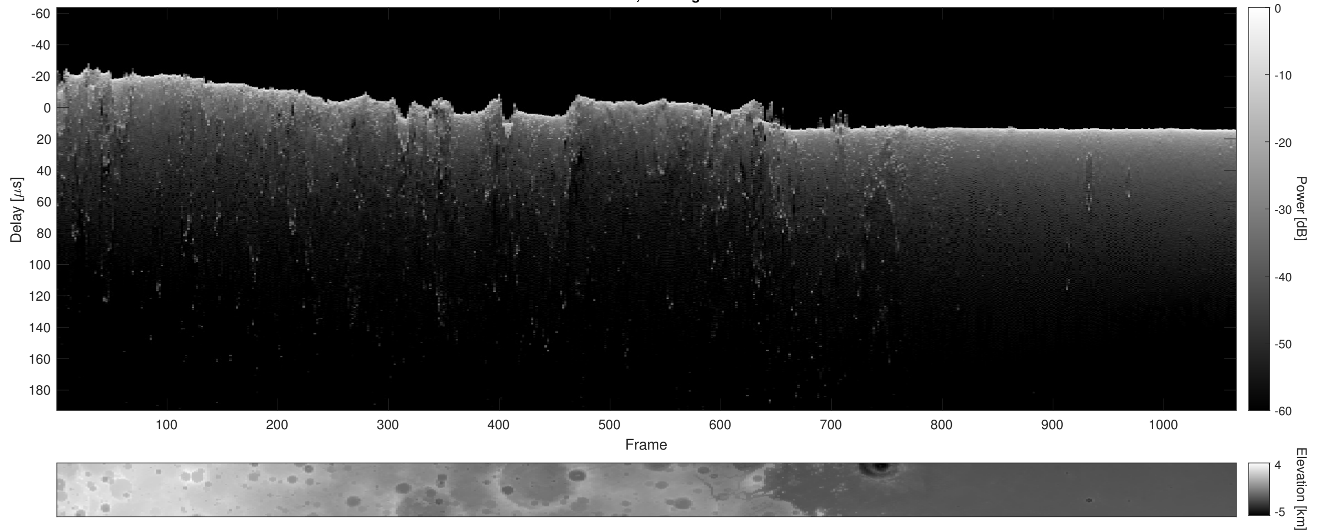
Orbit 5981, Cluttergram
