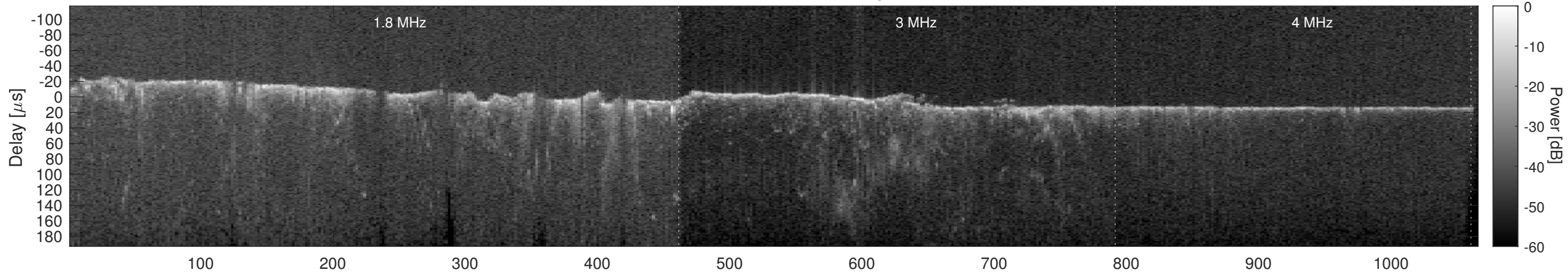
Orbit 5981, Cluttergram
