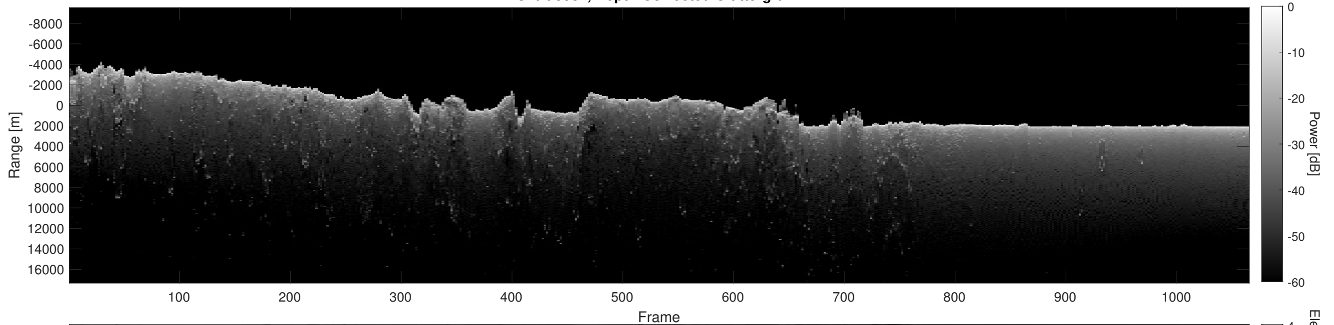
Orbit 5981, Depth-Corrected Cluttergram
