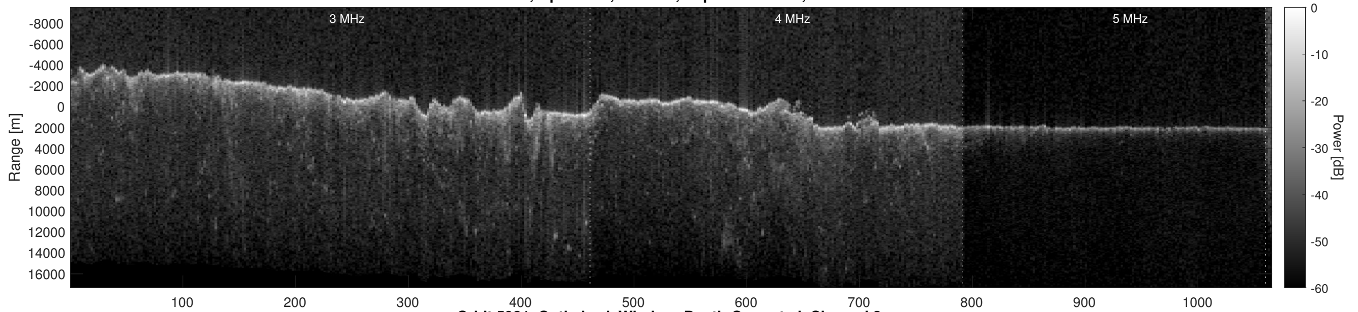
Orbit 5981, Optimized, Window, Depth-Corrected, Channel 2
