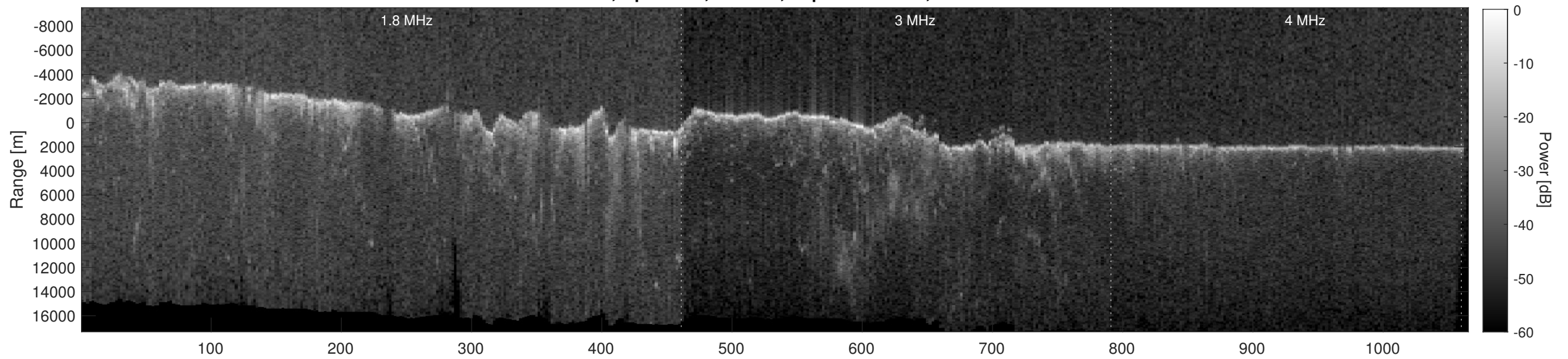
Orbit 5981, Depth-Corrected Cluttergram
