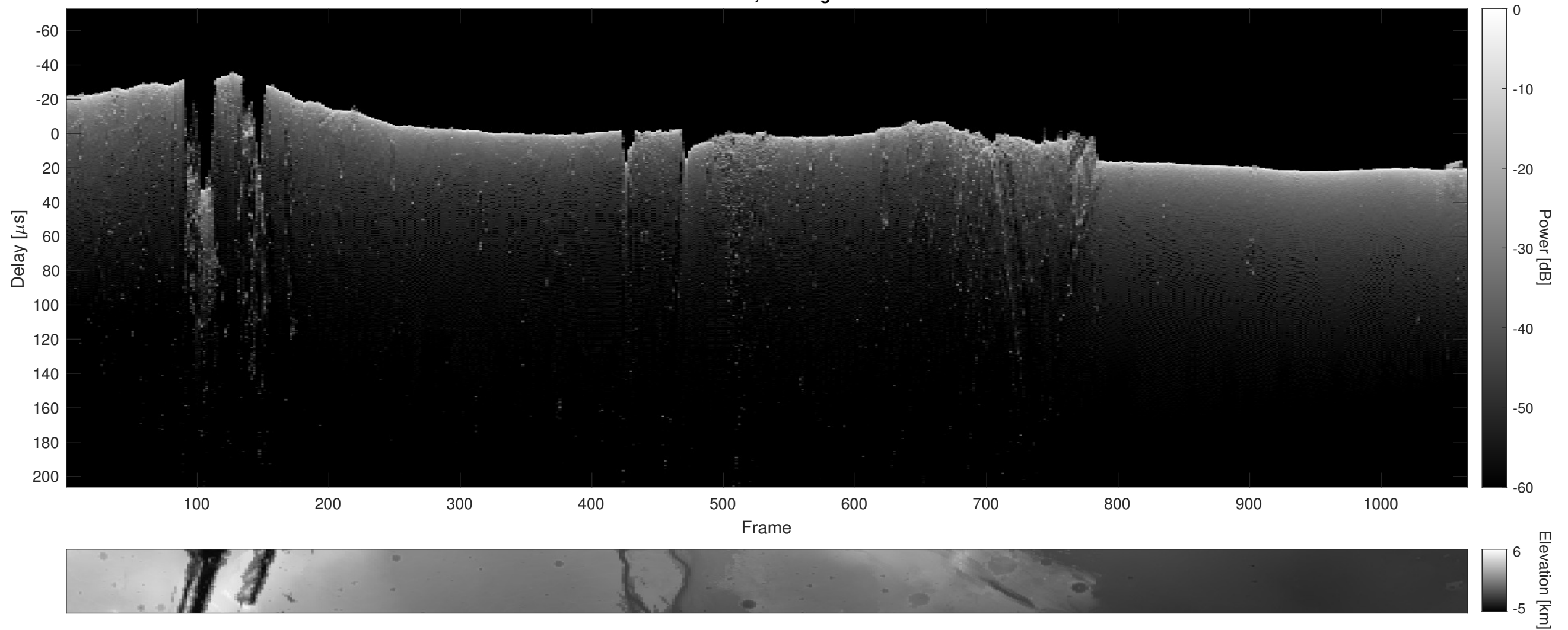
Orbit 5982, Cluttergram
