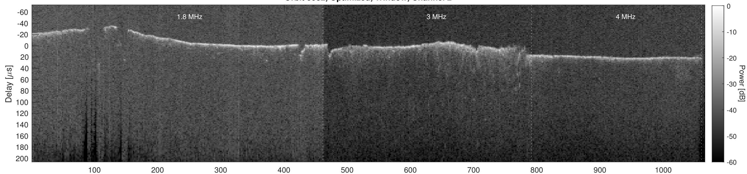
Orbit 5982, Cluttergram
