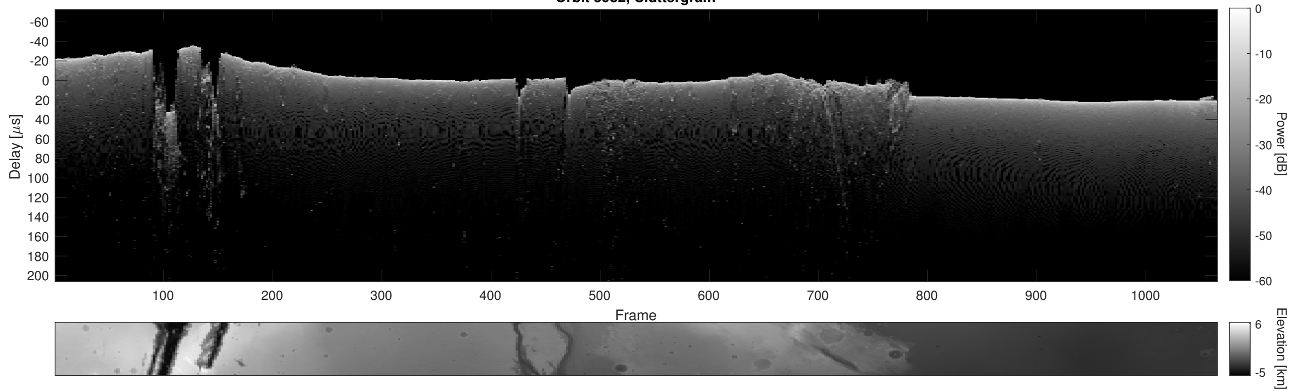
Orbit 5982, Cluttergram
