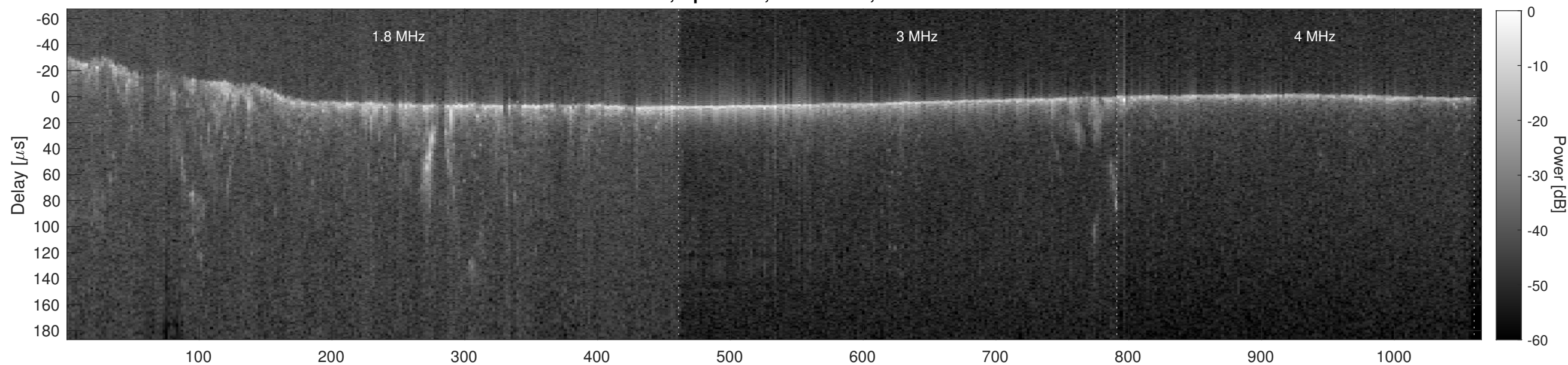
Orbit 5983, Cluttergram
