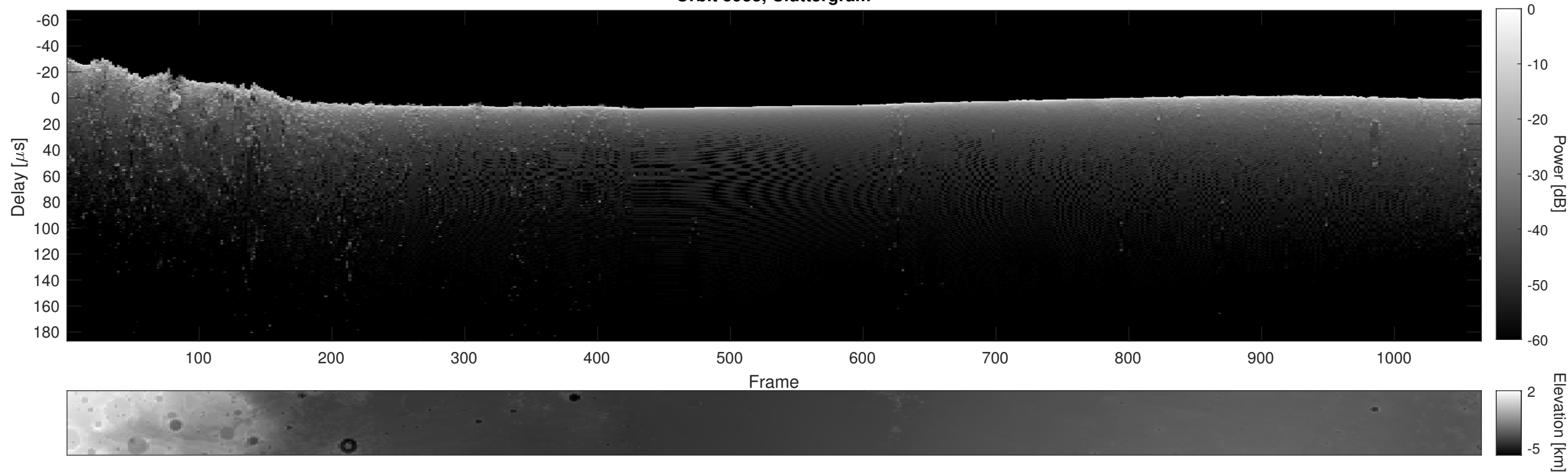
Orbit 5983, Cluttergram
