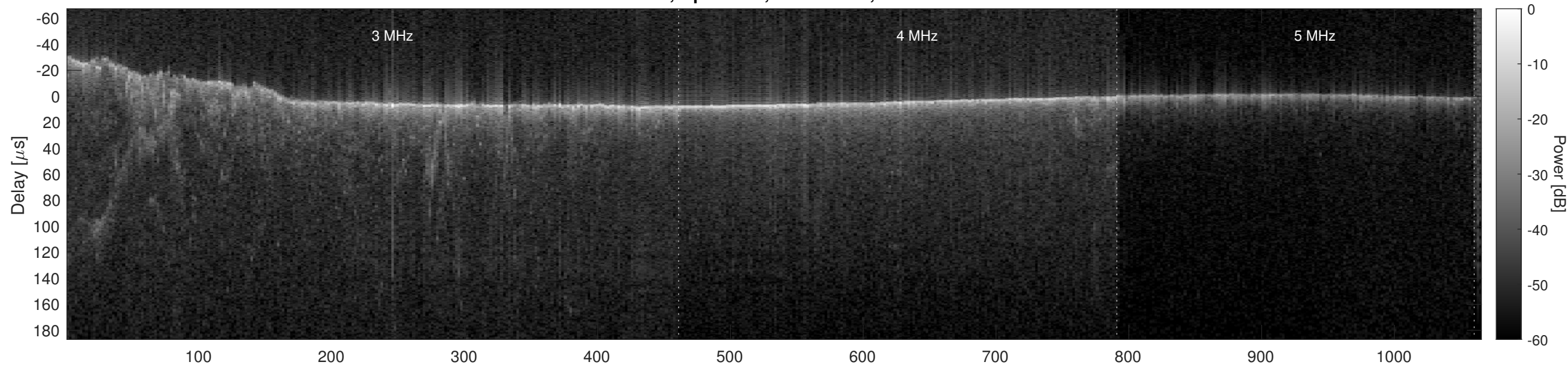
Orbit 5983, Optimized, No Window, Channel 2
