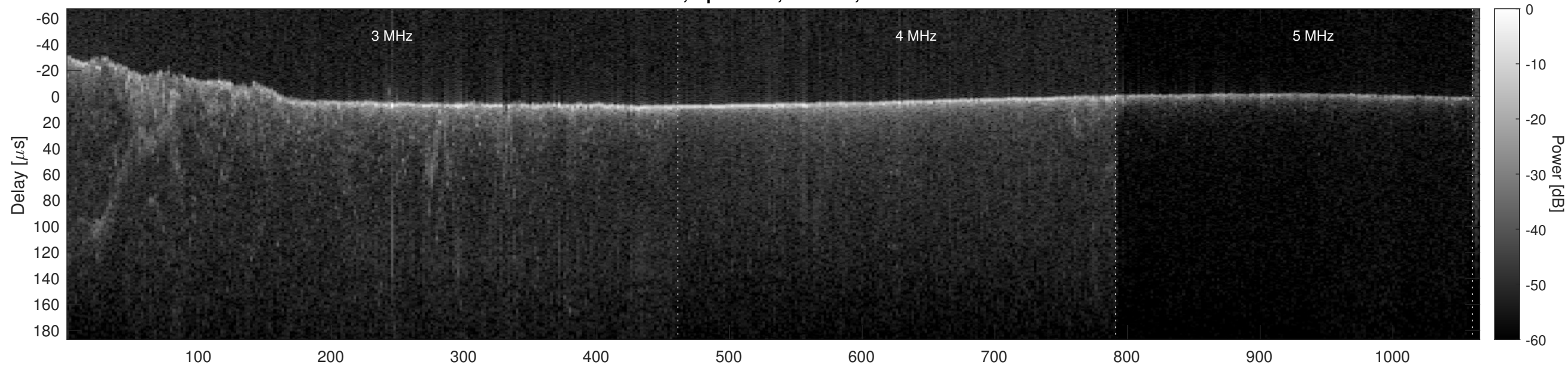
Orbit 5983, Optimized, Window, Channel 2
