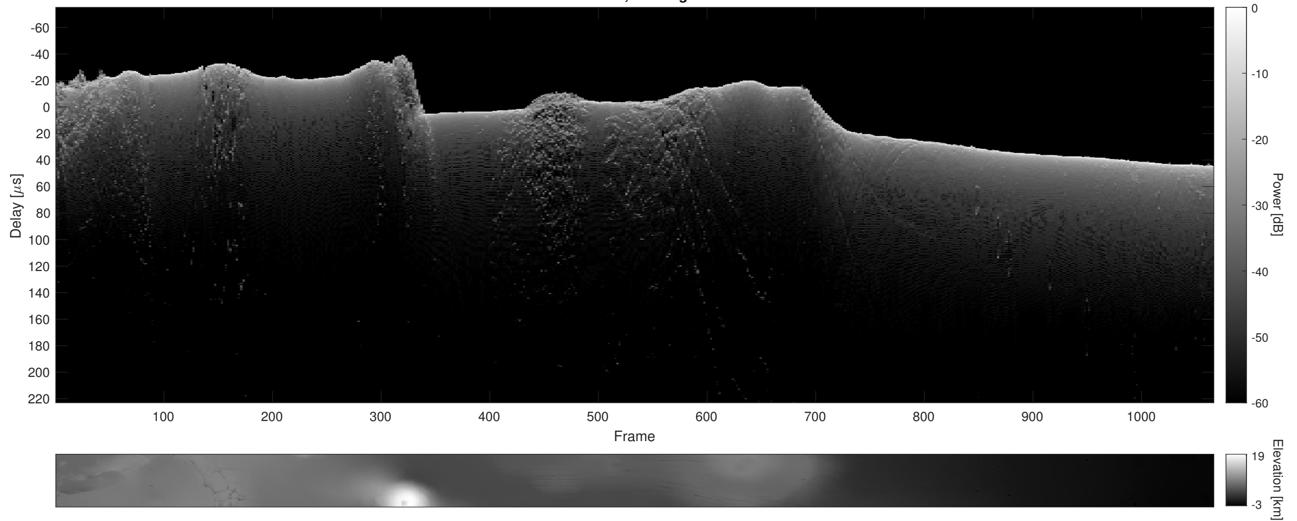
Orbit 5986, Cluttergram
