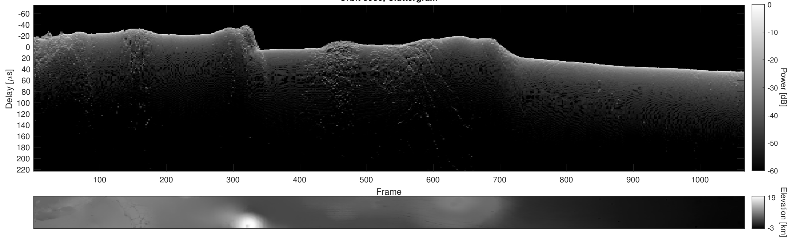
Orbit 5986, Cluttergram
