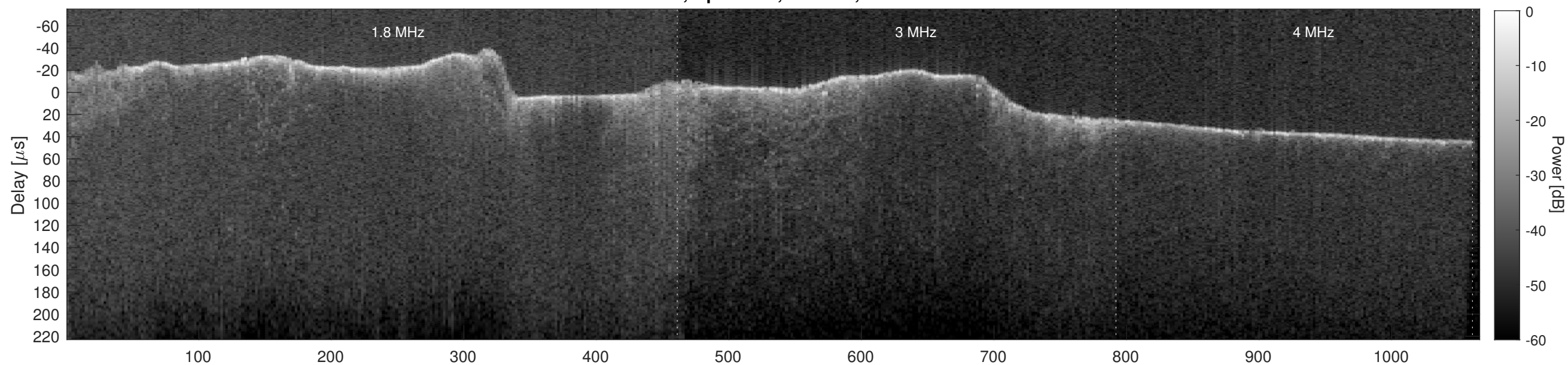
Orbit 5986, Cluttergram
