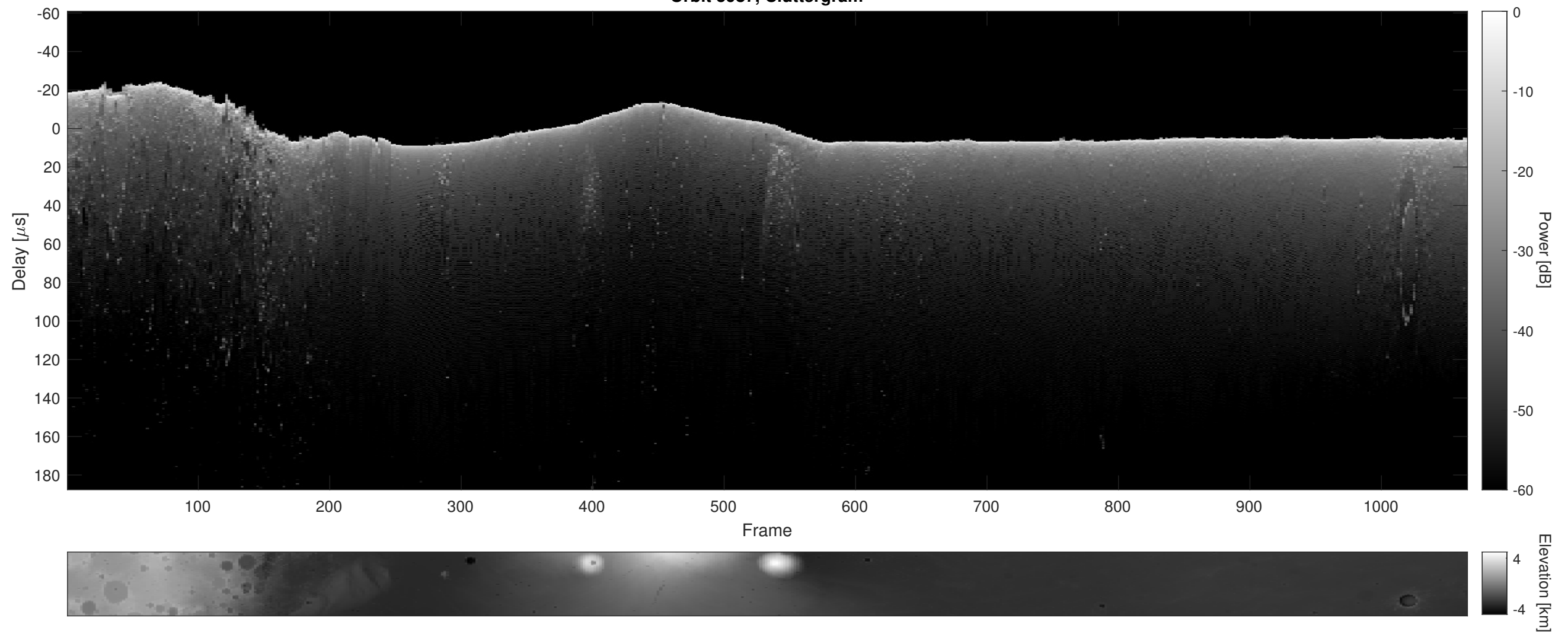
Orbit 5987, Cluttergram
